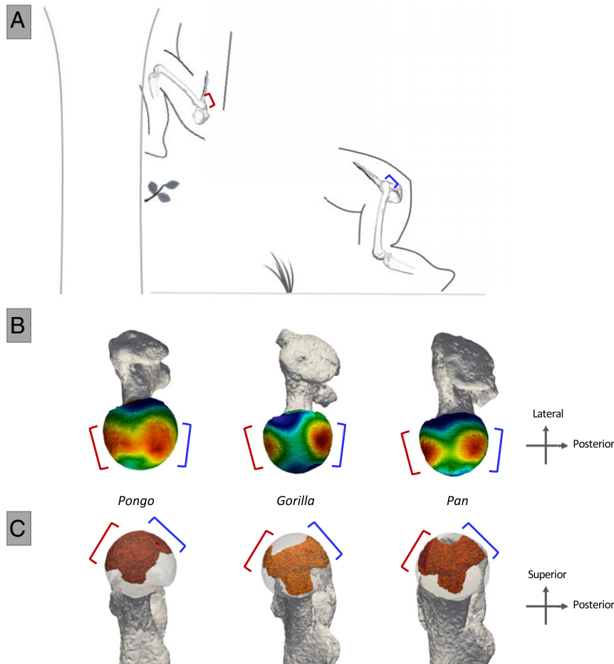
Fig. 2. Nonhuman great ape hip flexion angles during terrestrial vertical climbing and quadrupedalism, and BV/TV distribution in the femoral head. (A) Great ape hip posture in maximum flexion ( \sim 55^\circ to 60^\circ ) during climbing (39), as well as joint posture at toe-off ( \sim 110^\circ ) during terrestrial knuckle walking (40). Brackets indicate regions of presumed high pressure during large flexion (red, anterior) and slight flexion (blue, posterior). (B) Superior view of BV/TV distribution in the femoral head of Pongo , Gorilla , and Pan . High BV/TV is indicated in red and low BV/TV in blue. Note the two distinctly high BV/TV concentrations in Gorilla and the expansive distribution in Pongo , with Pan exhibiting an intermediate pattern. (C) Distribution of highest BV/TV values within the femoral head of Pongo , Gorilla , and Pan . Internal concentrations are visualized for BV/TV above the 80th percentile. This threshold was chosen to visualize the regions where the highest BV/TV is found within each specimen. Note that the internal high BV/TV forms an inverted cone in Pongo , and two convergent pillars in Pan and Gorilla .
