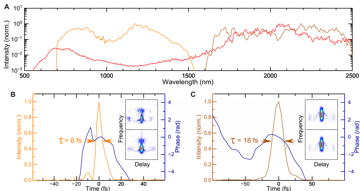
Fig. 2. The laser specifications. (A) CEP-stable, multi-octave spectrum of seed pulses (red). Amplified spectra of NIR (orange) and MIR (brown) OPCAs. Retrieved temporal intensity profile and phase of the compressed pulses in (B) NIR and (C) MIR channels. Inset: Measured (top) and retrieved (bottom) FROG spectrograms.
