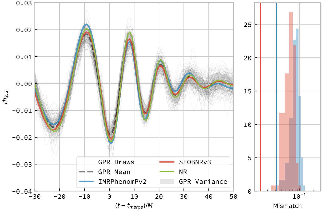
FIG. 7. GPR predictions, compared to NR. One hundred draws from the Gaussian process (left panel) for a non-spinning configuration ( \mathbf{s}_1 = (0, 0, 0) , \mathbf{s}_2 = (0, 0, 0) , \mathbf{q} = 0.625 ), shown as light grey lines compared to the phenomenological approximant models, IMRPhenomPv2 in blue; and SEOBNRv3 in red. The mean draw from the Gaussian process is shown as a grey dashed line, while the associated variance is plotted as a grey-filled region surrounding the mean. The differences between the phenomenological model and the GPR model waveforms are seen to also exist between the phenomenological model waveforms and the NR-derived waveform, plotted here in purple. In the right panel the distribution of mismatches between the samples and both phenomenological waveforms are shown, with the vertical lines representing the mismatch between the mean waveform from the GPR and each phenomenological waveform.
