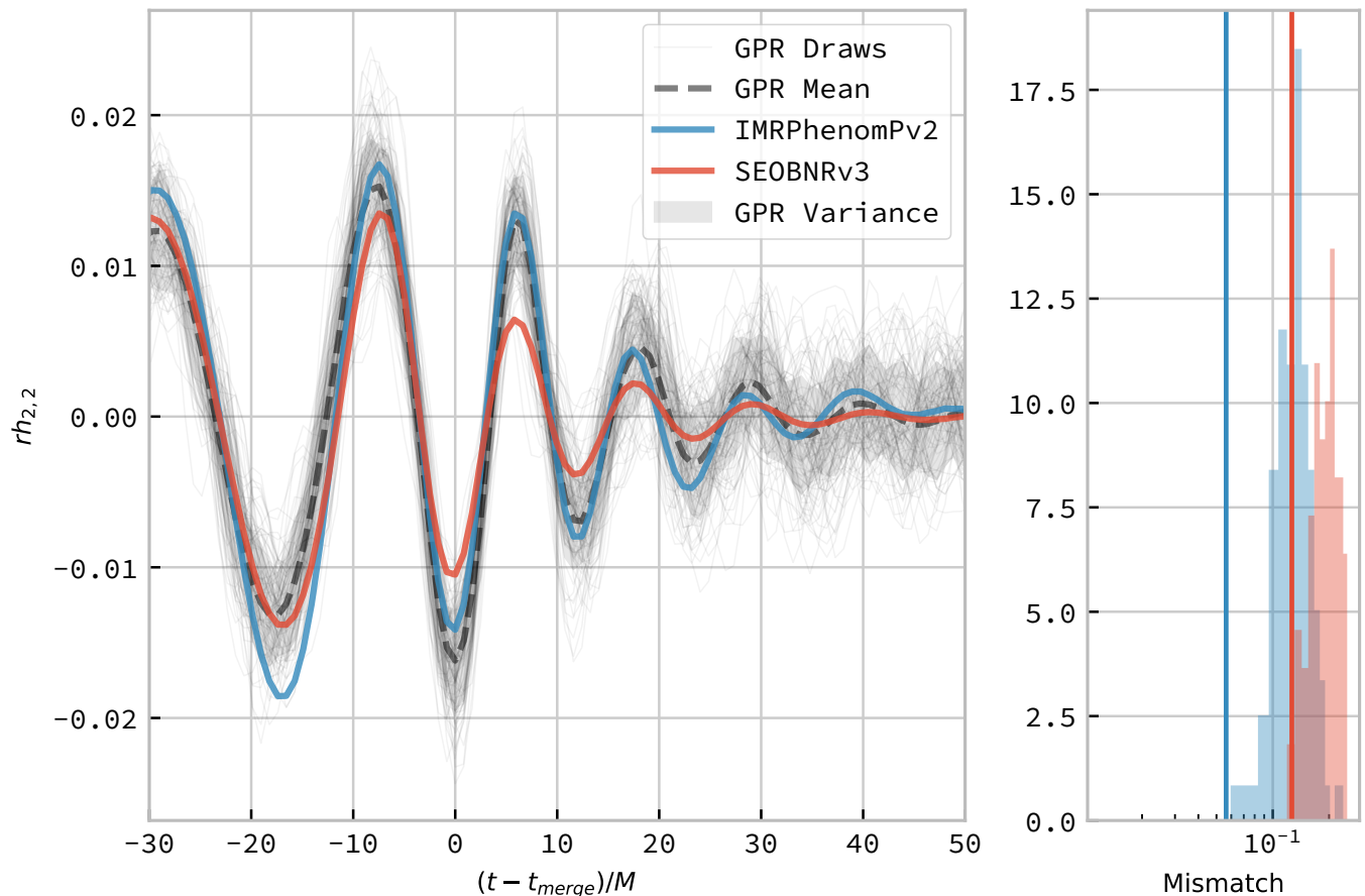
FIG. 6. Precessing waveform. One hundred draws from the Gaussian process (left panel) for a precessing system, with a mass ratio q = 0.4 , and a spin configuration ( \mathbf{s}_1 = (-0.5, -0.15, 0.3) , \mathbf{s}_2 = (0.5, 0.13, 0.3) ), shown as light grey lines compared to two phenomenological approximant models, SEOBNRv3 and IMRPhenomPv2 in red and blue respectively. The mean draw from the Gaussian process is shown as a grey dashed line, while the associated variance is plotted as a grey-filled region surrounding the mean. In the right panel the distribution of mismatches between the samples and both phenomenological waveforms are shown, with the vertical line representing the mismatch between the mean waveform from the GPR and the phenomenological waveform.
