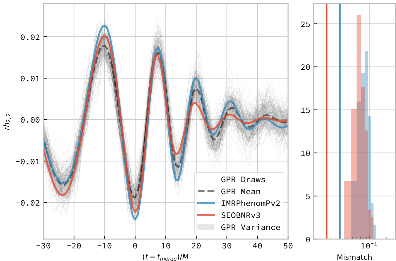
FIG. 5. Anti-aligned spin waveform. One hundred draws from the Gaussian process (left panel) for a non-spinning, equal-mass configuration ( \mathbf{s}_1 = (0, 0, 0.6) , \mathbf{s}_2 = (0, 0, -0.6) , \mathbf{q} = 1.0 ), shown as light grey lines compared to two phenomenological approximant models, SEOBNRv3 and IMRPhenomPv2 in red and blue respectively. The mean draw from the Gaussian process is shown as a grey dashed line, while the associated variance is plotted as a grey-filled region surrounding the mean. In the right panel the distribution of mismatches between the samples and both phenomenological waveforms are shown, with the vertical lines representing the mismatch between the mean waveform from the GPR and the phenomenological waveform.
