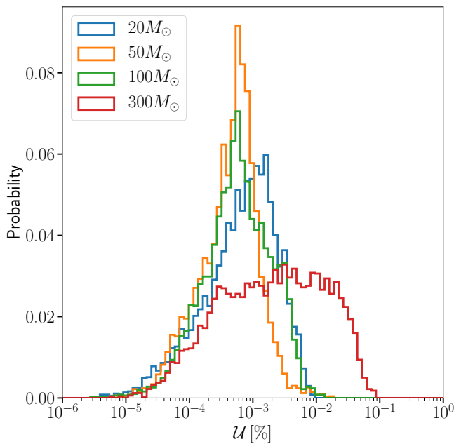
FIG. 4: Histograms of the unfaithfulness \bar{\mathcal{U}} (in percent) between SEOBNRv4HM and ROM waveforms for different values of the total mass.
