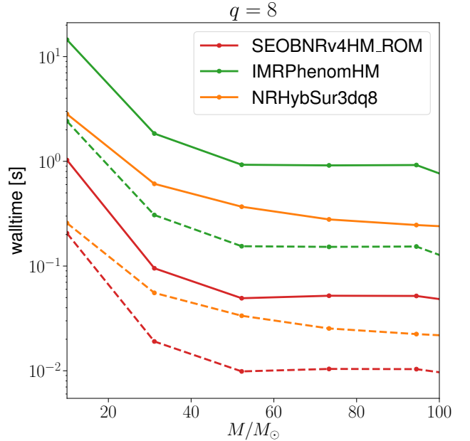
FIG. 9: Walltime comparison between different spin-aligned waveform models with higher-order modes as a function of the total mass and for q = 8 . The dashed lines indicate the walltime normalized by the number of modes included in the model respectively 5 for SEOBNRv4HM_ROM, 6 for IMRPhenomHM and 11 for NRHybSur3dq8.
