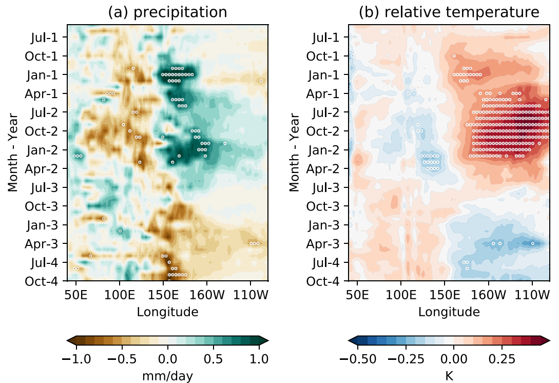
Figure 7. Indo-Pacific equatorial ( 5^{\circ} S– 5^{\circ} N) multimodel ensemble mean Hovmöller plots for (a) precipitation (mm/day) and (b) surface temperature relative to the tropics ( 20^{\circ} S– 20^{\circ} N, K). Stippling indicates significant values.
