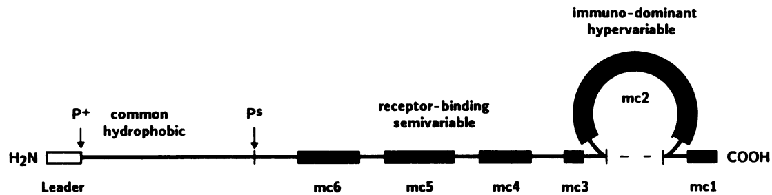
FIG. 1. Primary structure of propilin. Propilin consists of about 160 amino acids plus a seven-amino-acid leader. P + and P s denote alternative processing sites of propilin at positions 1 and 40, respectively. mc1 to mc6 indicate the minicassettes, i.e., the regions which differ in variant pilins and among silent and expressed pilin genes.
