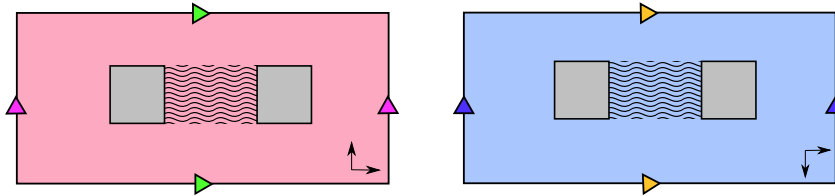
FIGURE 3. Good cylinder decomposition to deform \alpha_i
