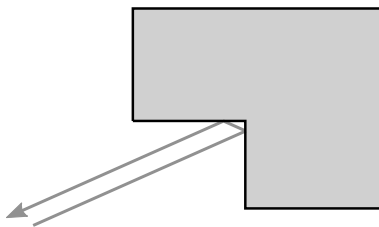
FIGURE 8. Flow bouncing close to a concave right angle.
