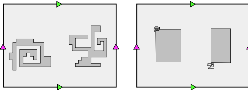
FIGURE 4. Example of deformation
