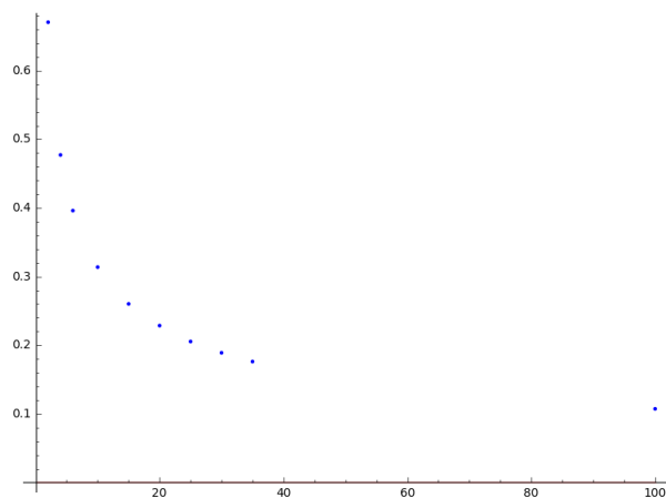
FIGURE 7. Principal Lyapunov exponent for \mathcal{Q}(1^{8+p}, -1^p)
