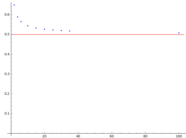
FIGURE 5. Principal Lyapunov exponent for \mathcal{Q}(1^{4n})
