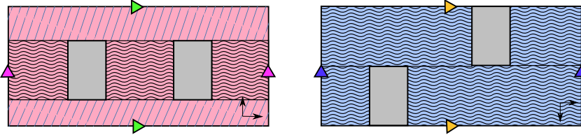
FIGURE 2. Good cylinder decomposition to deform b_1
