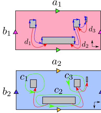
FIGURE 1. Basis for relative homology.
