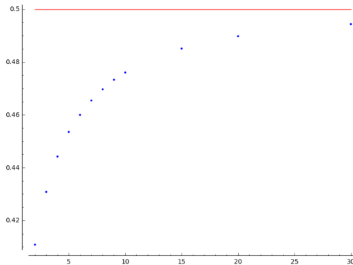
FIGURE 6. Principal Lyapunov exponent for \mathcal{Q}(1^{4n+10}, -1^{10})
