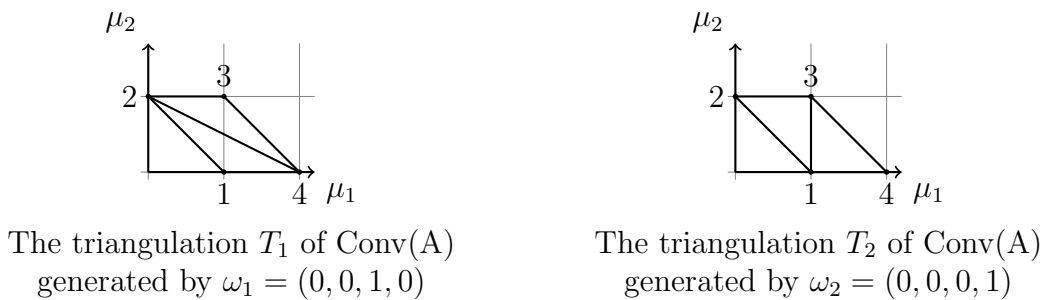
Figure 2: The two possible regular triangulations of the Newton polytope \Delta_G = \text{Conv}(A) corresponding to the Lee-Pomeransky polynomial G = z_1x_1 + z_2x_2 + z_3x_1x_2 + z_4x_1^2 .
