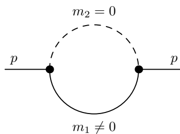
Figure 1: The 1-loop 2-point function with one mass.
