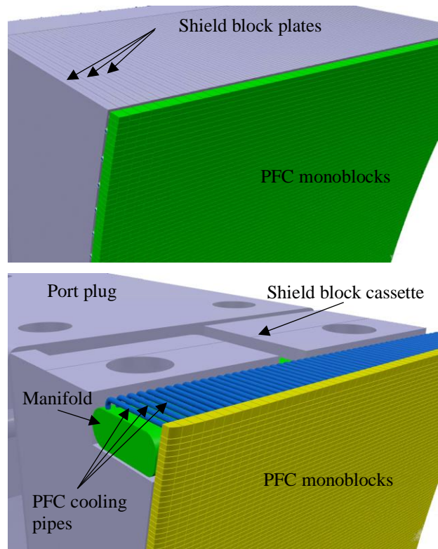
Figure 5: Upper left corner of Outboard Mid-plane Limiter: above, plate-based design below, divertor-like design.
