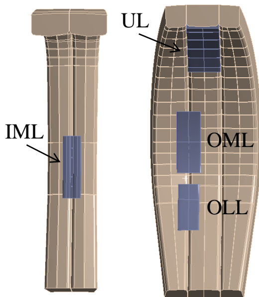
Figure 4: Limiters in a sector: left, inboard view, right, outboard view (without PFCs).
