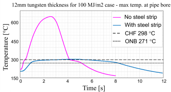
Figure 3: Comparison of pipe bore peak temperature with and without thermal break for 12 mm tungsten monoblock thickness.
