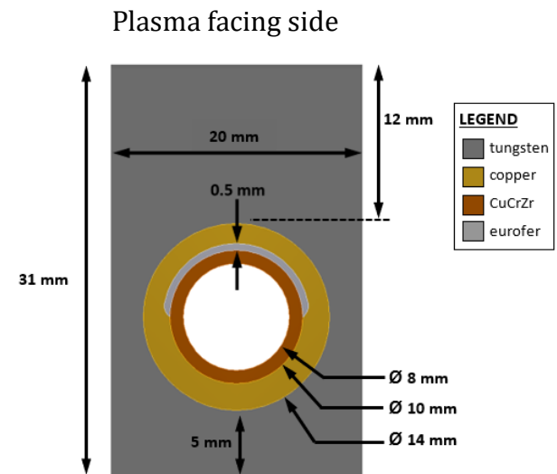
Figure 2: Monoblock cross-section for upper limiter.
