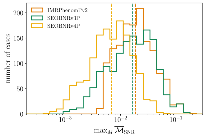
FIG. 8. Sky-and-polarization averaged, SNR weighted unfaithfulness for an inclination \iota = \pi/3 between NR waveforms with \ell = 2 and SEOBNRv4P , and also SEOBNRv3P and IMRPhenomPv2 , which were used in LIGO/Virgo publications. The vertical dashed lines show the medians. It is evident the better performance of the newly developed precessing model SEOBNRv4P .
