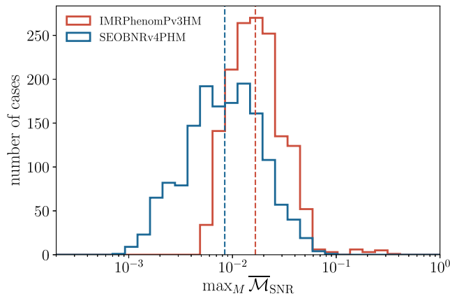
FIG. 13. The highest unfaithfulness over total mass for all cases shown in Fig. 12. The median of unfaithfulness is around 1% for SEOBNRv4PHM and 2% for IMRPhenomPv3HM (shown as dashed vertical lines). Note that for SEOBNRv4PHM, the worst unfaithfulness is below 10% and the distribution is shifted to lower values.
