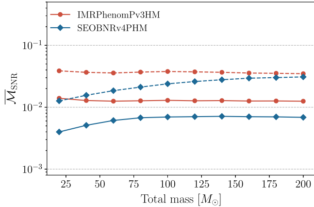
FIG. 12. Summary of unfaithfulness as a function of the total mass, for all NR simulations considered as shown in Fig. 10 and Fig. 11. The solid (dotted) line represents the median (95th-percentile) of all cases. For all total masses, we find that the median mismatch with SEOBNRv4PHM is lower than 1%, about a factor of 2 lower than IMRPhenomPv3HM. The 95th-percentile shows a stronger dependence on total mass for SEOBNRv4PHM, with mismatches lower than IMRPhenomPv3HM at low and medium total masses, becoming comparable at the highest total masses.
