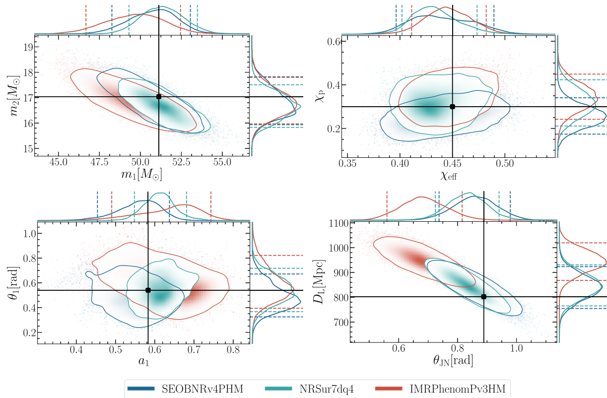
FIG. 15. 2D and 1D posterior distributions for some relevant parameters measured from the first synthetic BBH signal with mass ratio q = 3 , total source-frame mass of M = 70 M_{\odot} , spins of the two BHs \chi_1 = (0.30, 0.00, 0.50) and \chi_2 = (0.20, 0.00, 0.30) defined at a frequency of 20 Hz. The inclination with respect to the line of sight of the BBH is \iota = \pi/3 . The other parameters are specified in the text. The signal waveform is generated with the waveform model NRSur7dq4. In the 2D posteriors, solid contours represent 90% credible intervals and black dots show the value of the parameter used in the synthetic signal. In the 1D posteriors they are represented respectively by dashed lines and black solid lines. The parameter estimation is performed with the waveform models SEOBNRv4PHM (blue), NRSur7dq4 (cyan), and IMRPhenomPv3HM (red). Top left: component masses in the source frame, Top right: \chi_{\text{eff}} and \chi_p , Bottom left: magnitude and tilt angle of the primary spin, Bottom right: \theta_{\text{JN}} and luminosity distance.
