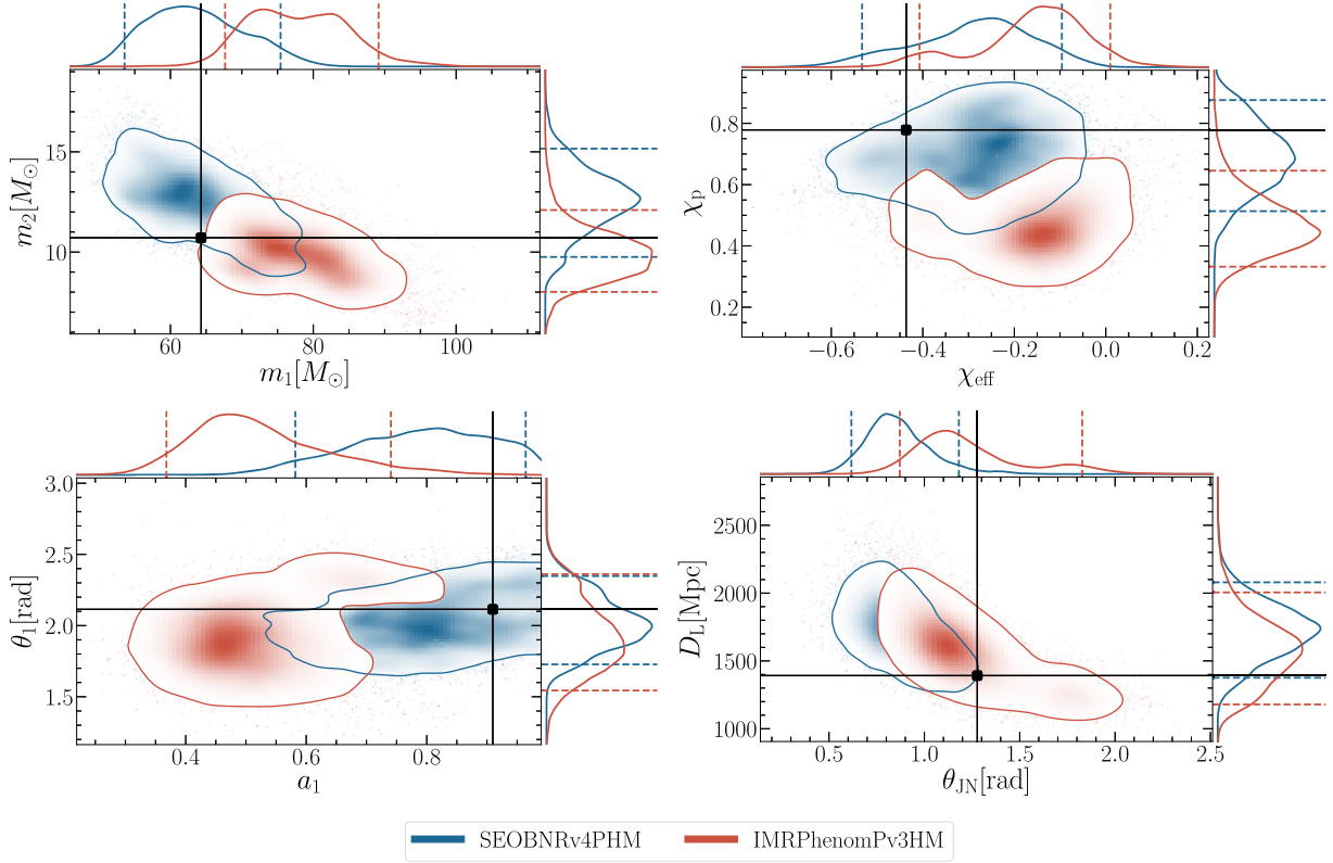
FIG. 16. 2D and 1D posterior distributions for some relevant parameters measured from the first synthetic BBH signal with mass ratio q = 6 , total source-frame mass of M = 76 M_{\odot} , spins of the two BHs \chi_1 = (-0.06, 0.78, -0.47) and \chi_2 = (0.08, -0.17, -0.23) defined at a frequency of 20 Hz. The inclination with respect to the line of sight of the BBH is edge-on, i.e., i = \pi/2 . The other parameters are specified in the text. The signal waveform is generated using the NR waveform from the SXS public catalog SXS:BBH:0165. In the 2D posteriors solid contours represent 90% credible intervals and black dots show the value of the parameter used in the synthetic signal. In the 1D posteriors they are represented respectively by dashed lines and black solid lines. The parameter estimation is performed with the waveform models SEOBNRv4PHM (blue) and IMRPhenomPv3HM (red). Top left: component masses in the source frame, Top right: \chi_{\text{eff}} and \chi_p , Bottom left: magnitude and tilt angle of the primary spin, Bottom right: \theta_{\text{JN}} and luminosity distance.
