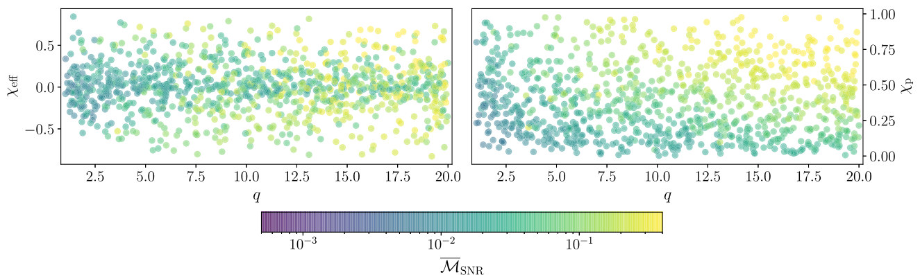
FIG. 14. Sky- and polarization-averaged unfaithfulness between SEOBNRv4PHM and IMRPhenomPv3HM for 1000 random configurations. Notice that the unfaithfulness grows both with the mass ratio and the spin and can reach very large values for q \approx 20 and high \chi_p . It is also clear that for cases with smaller spins the unfaithfulness remains much lower.
