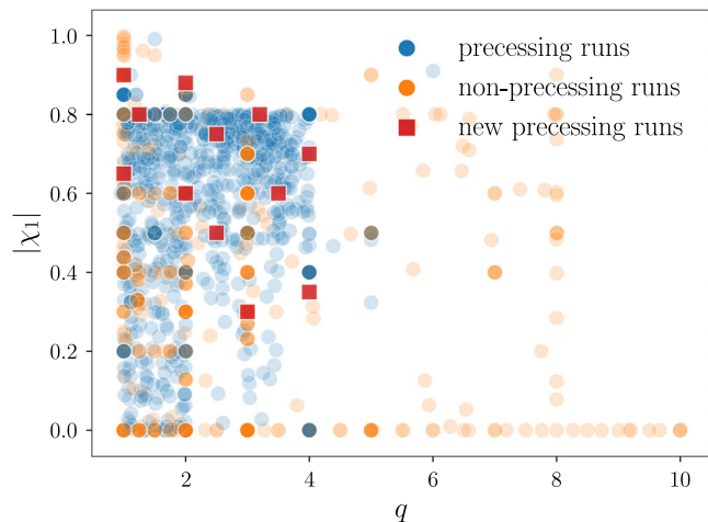
FIG. 1. Parameter space coverage in q - \chi_1 space for SpEC waveforms. For runs from the SpEC catalog [57] the opacity was changed so that runs with similar parameters are clearly visible. We indicate with squares precessing BBH runs performed as part of this paper.
