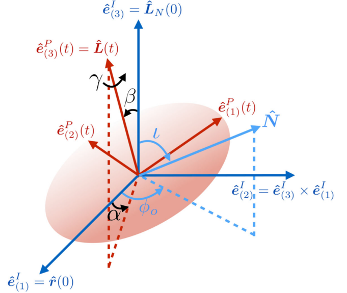
FIG. 5. Frames used in the construction of the SEOBNRv4 PHM model: the observer's frame (blue), defined by the directions of the initial orbital angular momentum \hat{\mathbf{L}}(0) and separation \mathbf{r}(0) , and coprecessing frame (red), instantaneously aligned with \hat{\mathbf{L}}(t) and described by the Euler angles (\alpha, \beta, \gamma) (see text below for details).
