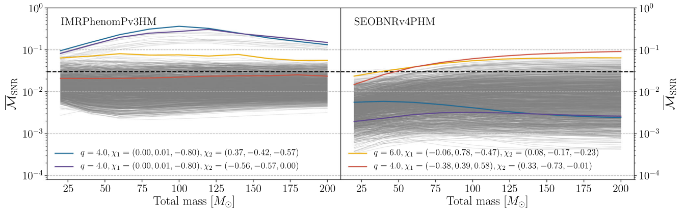
FIG. 10. The sky-and-polarization averaged, SNR-weighted unfaithfulness as a function of binary's total mass for inclination \iota = \pi/3 , between IMRPhenomPv3HM and NR (left) and SEOBNRv4PHM and NR (right) for 1404 quasi-circular precessing BBH simulations in the SXS public catalog. The colored lines highlight the cases with the worst maximum mismatches for both models. Note that for the majority of cases, both models have unfaithfulness below 5%, but SEOBNRv4PHM has no outliers beyond 10% and many more cases at lower unfaithfulness.
