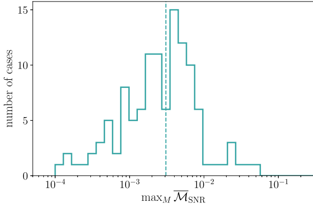
FIG. 2. The sky-and-polarization-averaged unfaithfulness between the highest and second highest resolutions in the NR simulation maximized over the total mass for the new 118 NR precessing waveforms. The inclination used is \pi/3 . The vertical dashed line shows the median.
