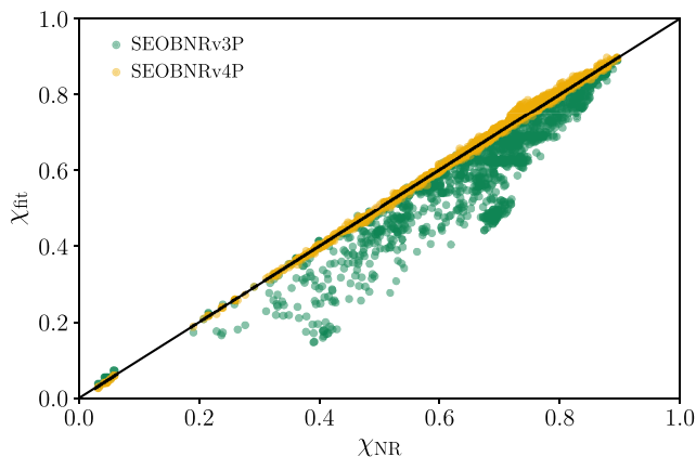
FIG. 6. Comparison of the magnitude of the final spin between the SEOBNRv3P and SEOBNRv4P models and NR results. For simplicity, the fits are evaluated using the NR data at the relaxed time. The black line is the identity. It is obvious that SEOBNRv4P gives final-spin magnitudes much closer to the NR values.
