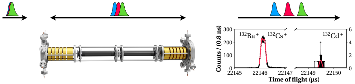
Figure 2.2: Left: Schematic diagram of the ISOLTRAP MRToF mass spectrometer/separator. Beam composed of different species with well-defined energy enters the device at the left and is trapped for a certain number of revolutions N_{\text{rev}} (typically N_{\text{rev}} = 1 \times 10^3 at ISOLTRAP). There, ions undergo a time-of-flight separation, and their time of flight can be measured. Right: Time-of-flight spectrum of ^{132}\text{Cd}^+ with a mass resolving power of m/\Delta m \sim 1 \times 10^5 .
