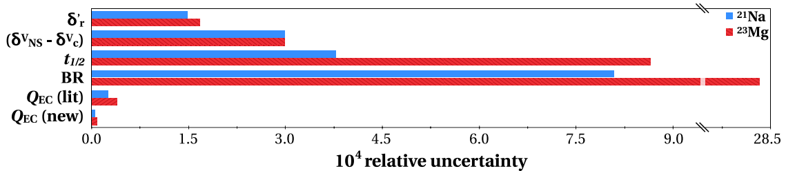
FIG. 6. Comparison of the relative uncertainty contributions to the \mathcal{F}t^{\text{mirror}} value: the nucleus-dependent radiative corrections, \delta'_r , and \delta^{V_{NS}} , the isospin-symmetry-breaking corrections \delta^{V_C} , the half-lives, the branching ratios BR, and the Q_{EC} values from Ref. [16] for ^{21}\text{Na} (blue), from Ref. [15] for ^{23}\text{Mg} (red), as well as from this work. For details, see text.
