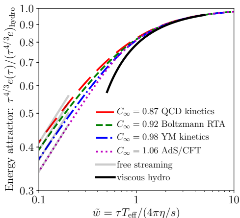
FIG. 24. Hydrodynamic attractors for pre-equilibrium evolution of energy density for different microscopic theories. From [42].
