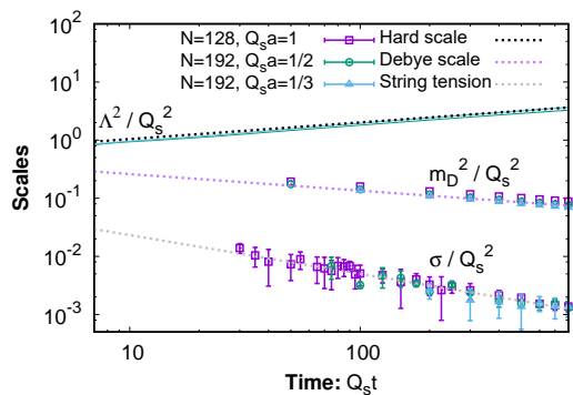
FIG. 16. Time evolution of the hard scale ( \Lambda^2 ), the electric screening scale ( m_D^2 ), and the spatial string tension ( \sigma ). Symbols for m_D^2 and \sigma denote lattice results for the different lattice spacings employed, while the solid green line represents a continuum extrapolation for the hard scale. The dotted lines represent perturbative estimates for the hard and Debye scales, and a fit to the lattice results for the non-perturbative string tension scale. From Ref. [322].
