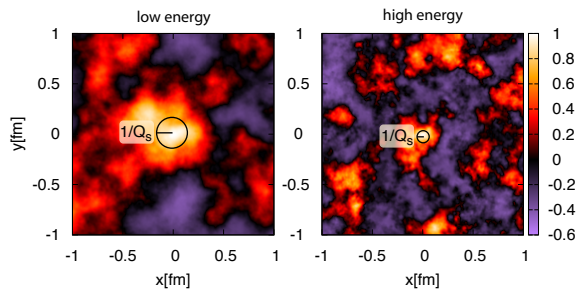
FIG. 4. Solution of the JIMWLK equation for the correlator of Wilson lines V(x_\perp)V^\dagger(y_\perp) probed by the DIS dipole [174]. As the nucleus is boosted from low energy (or rapidity) to high energy, the regions with large values of these correlator shrink spatially, corresponding to larger values of Q_s .
