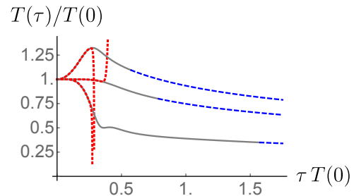
FIG. 27. Evolution of the effective temperature as a function of time for three different states with nonzero initial energy density. The gray curves denote the far-from-equilibrium regime. The blue dashed area extending indefinitely to the right mark the applicability of viscous hydrodynamic relations truncated at the third order in derivatives (122). The red dotted curves denote the series in Eq. (120) extracted using the method of Ref. [489]. Adapted from Ref. [479].
