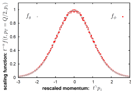
FIG. 14. The normalized distribution for the scalar theory f_\phi as a function of the rescaled longitudinal momentum at different times in the self-similar regime compared to the gauge theory f_g . From Ref. [52].
