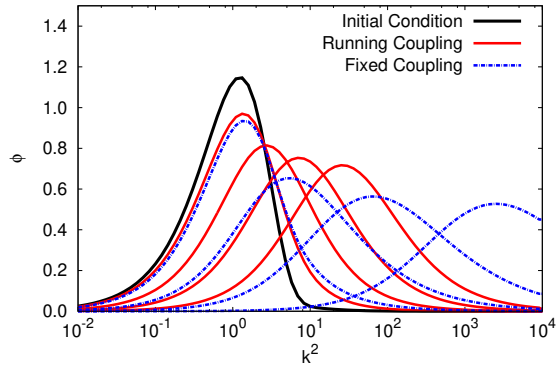
FIG. 3. Unintegrated gluon distribution (in units of the transverse area) vs the squared transverse momentum (normalized to its value at the peak of the initial condition curve) from the solution of the Balitsky-Kovchegov equation. The different curves represent increasing rapidities (left to right) for fixed and running coupling. From [151].
