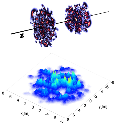
FIG. 8. Top panel: collisions of nuclei with sub-nucleon color charge fluctuations determined by the IP-Sat model. Bottom panel: the LO energy density in the Glasma at \tau = 1/Q_S . From [238].
