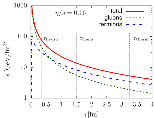
FIG. 25. Energy density evolution in a chemically equilibrating quark-gluon plasma. The vertical lines indicate the times of approximate hydrodynamic, chemical and thermal equilibriums. From Ref. [43].
