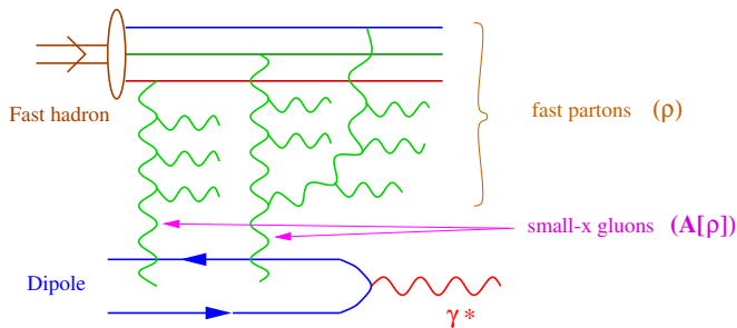
FIG. 2. DIS in the dipole picture. The virtual photon emitted by the electron splits into a q\bar{q} dipole that scatters off dynamical small x gauge fields coupled to the static large x lightcone sources. From [110].
