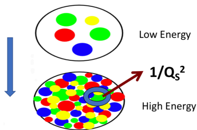
FIG. 1. Transverse hadron profile resolved in scattering with fixed squared momentum transfer Q^2 and increasing center-of-mass energy \sqrt{s} . The requirement for proliferating soft gluons to have maximal occupancy 1/\alpha_S generates the close packing saturation scale Q_S . Adapted from [110].
