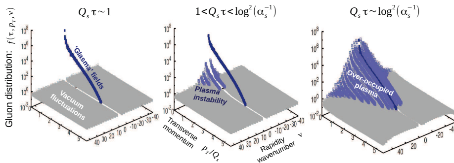
FIG. 10. Time evolution of the gluon distribution at early times 0 \lesssim Q_s \tau \lesssim \log^2(\alpha_s^{-1}) from next-to-leading order CGC initial conditions [264] at very weak coupling ( \alpha_s \sim 10^{-6} ). From Ref. [298].
