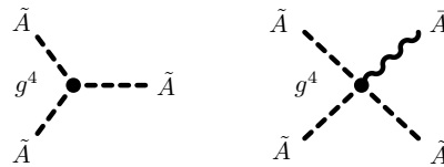
FIG. 18. Illustration of rescaled “quantum” three- and four-vertices, that are \sim g^4 . From Ref. [284].
