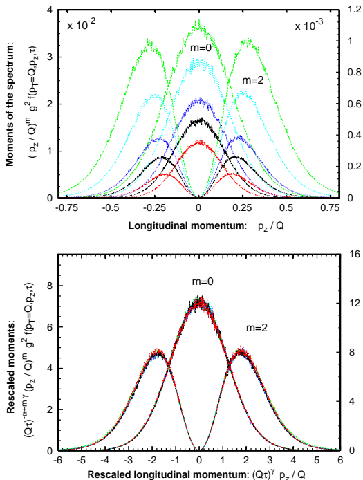
FIG. 13. Left panel: moments of the single particle distribution function as a function of longitudinal momenta. The longitudinal spectra are evaluated at transverse momentum p \simeq Q . The different curves correspond to different times of the evolution: Q\tau = 750, 1000, 1500, 2000, 3000 (from top to bottom). Right panel: the rescaled moments of the distribution function are found to collapse onto a single curve when plotted as a function of the rescaled longitudinal momentum variable. From Ref. [27].
