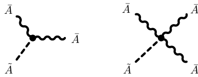
FIG. 17. Illustration of rescaled “classical” three- and four-vertices, that are independent of the coupling. From Ref. [284].
