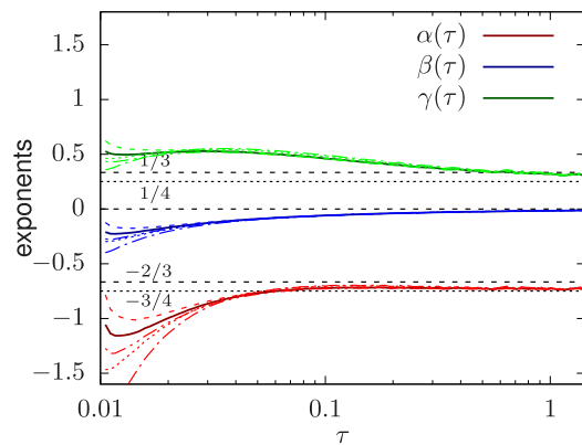
FIG. 21. Time evolution of instantaneous scaling exponents extracted from different sets of integral moments of the distribution. Horizontal lines indicate possible asymptotic values. From Ref. [428].
