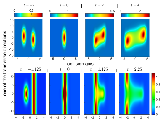
FIG. 31. Energy density in holographic heavy-ion collisions with transverse dynamics. Top panels: off-central collision with modest elliptic flow. Bottom panels: proton-nucleus collision as modeled with a shockwave with a small Gaussian extent in the transverse plane (left projectile) and a planar shock (right projectile). The smaller projectile punches out a hole in the larger projectile and excites matter at mid-rapidity, leading to substantial radial flow. Adapted from [537] and [538].
