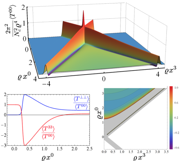
FIG. 30. \langle T^{\mu\nu} \rangle resulting from a collision of thin planar shocks with \varrho d = 0.08 (124). Top panel: lab-frame energy density as a function of time x^0 and longitudinal position x^3 . Between the remnants and the central rapidity region, there are small regions of negative energy density. Bottom-left panel: at mid-rapidity, the transverse and longitudinal pressure after the collision are consistent with \langle T^{00} \rangle \sim \tau^2 in Eq. (120). Bottom-right panel: the color encoding denotes deviations from constitutive relations and points to the applicability of hydrodynamics. The post-collision \langle T^{\mu\nu} \rangle does not have a rest frame in the gray region [543]. Adapted from Ref. [24].
