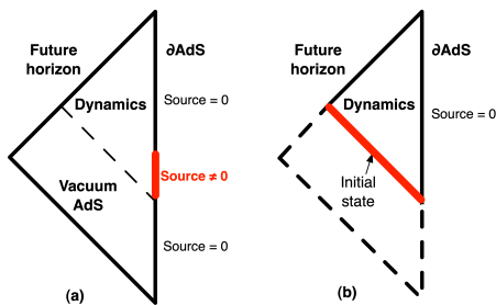
FIG. 26. Penrose diagrams dual to far-from-equilibrium states in strongly coupled QFTs. (a) The system starts in the vacuum with known bulk geometry and is perturbed by a non-trivial source, which appears as an asymptotic boundary condition in gravity. After the source is turned off, the QFT is in a non-equilibrium state modeled by a time dependent geometry. (b) The sources are always off, but one instead specifies non-trivial initial conditions for the bulk metric. Adapted from Ref. [482].
