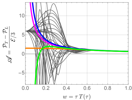
FIG. 28. \langle T^{\mu\nu} \rangle in a holographic CFT as a function of the dimensionless clock variable w for 29 different initial states (gray curves). Magenta, blue and green curves denote predictions of hydrodynamic constitutive relations truncated, respectively, at first, second, and third order [Eq. (122)]. The orange curve is the hydrodynamic attractor [30]. Adapted from Refs. [30, 47, 479].
