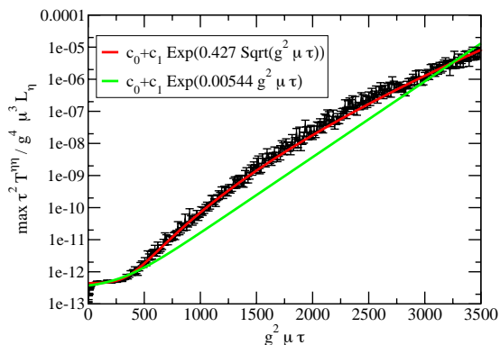
FIG. 9. Growth of the maximally unstable Fourier mode of the longitudinal pressure P_L = \tau^2 T^{\eta\eta} . Note that since g^2 \mu \propto Q_S , the results are in units of Q_S^3/g^2 , with g \sim 10^{-5} and L_\eta = 1.6 . From [41].
