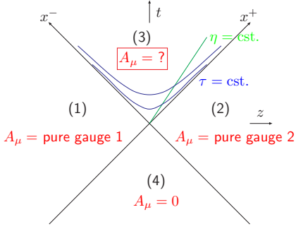
FIG. 6. Spacetime diagram of gauge field configurations. Before the collision, the gauge fields are pure gauge solutions with zero field strength. (In the text, the pure gauge solution of the right moving nucleus is denoted by A_{1,\text{cl.}}^i and that of the left moving nucleus is denoted by A_{2,\text{cl.}}^i .) After the collision, the gauge field solution ( \mathcal{A}^{i,\eta} in the text) correspond to finite field strengths in the Glasma. From [32].
