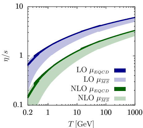
FIG. 22. The shear viscosity over entropy ratio as a function of temperature at leading (LO) and (nearly) next to leading order (NLO) thermal QCD. The bands correspond to the scale variation of running coupling prescriptions. Figure taken from [408].
