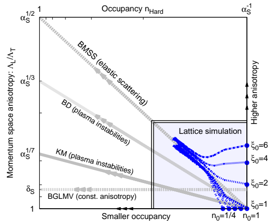
FIG. 12. Evolution in the occupancy–anisotropy plane, from Ref. [27]. Indicated are the thermalization scenarios proposed in (BMSS) [276], (BD) [277], (KM) [311] and (BGLMV) [312]. The blue lines show the results of classical-statistical simulations for different initial conditions [27, 298].
