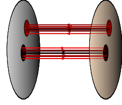
FIG. 7. Glasma flux tubes: Boost invariant LO Glasma configurations of transverse size 1/Q_S at \tau = 0^+ with parallel E_\eta and B_\eta , corresponding to finite Chern-Simons charge. Such configurations decay rapidly and are unstable to quantum fluctuations. From [230].
