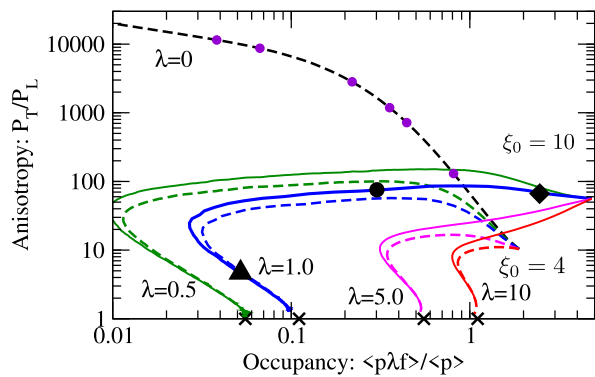
FIG. 20. Gluon kinetic theory equilibration in anisotropy-occupancy plane for initial anisotropy \xi_0 = 10 and different values of the coupling constant. Times corresponding to \tau Q_S = 10^0, 10^1, 10^3 are indicated by black symbols. Simulations with the smaller initial anisotropy \xi_0 = 4 are shown as dashed curves. Adapted from Ref. [381].
