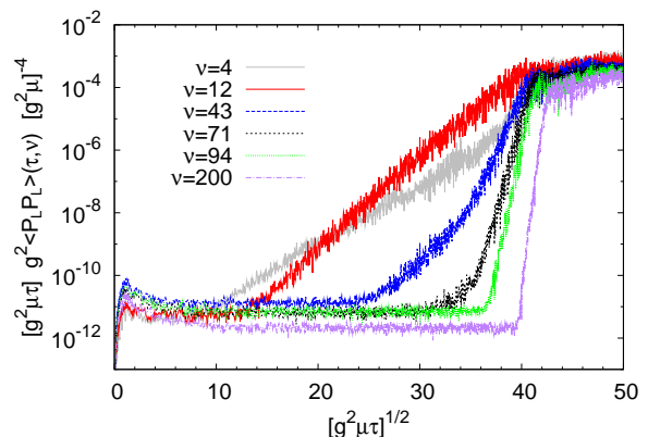
FIG. 11. Time evolution of the longitudinal pressure-pressure correlator for different rapidity wave numbers \nu with the parameters described in Ref. [272]. Once the initial fluctuations have grown larger, one observes the emergence of secondary instabilities at larger \nu with enhanced growth rates.
