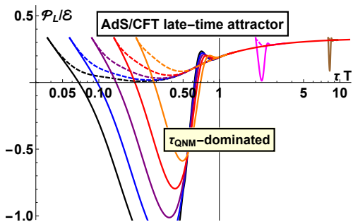
FIG. 29. Hydrodynamization of states whose gravity dual initially has support close to the boundary (dashed curves) or deep in the bulk (solid curves) initialized at different times (different colors); see the text for details. Adapted from Ref. [469].
