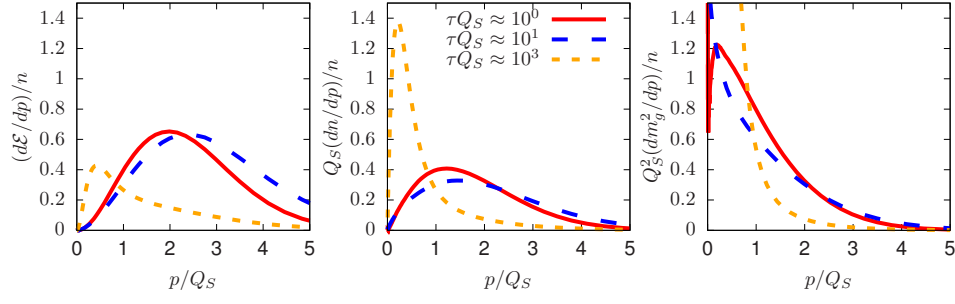
FIG. 19. Momentum differentiated plots of the (a) energy density (b) number density and (c) screening-mass at different stages of bottom-up thermalization. All curves are normalized by the instantaneous number density n and lines correspond to different times ( \tau Q_S = 10^0, 10^1, 10^3 ).
