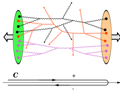
FIG. 5. Top panel: multi-particle production from cut “vacuum-vacuum” graphs connecting time dependent sources of the two nuclei after the collision. From [37]. Bottom panel: the Schwinger-Keldysh closed time contour on which the sources and fields are defined.
