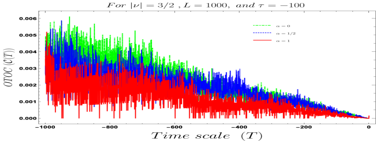
Figure 11: Behaviour of the four-point OTOC with respect to the T time scale of the theory. Here we fix, mass parameter \nu = -3i/2 , cut-off scale L = 1000 , vacuum parameter \alpha = 0 (Bunch Davies vacuum), 1/2 ( \alpha vacua), 1 ( \alpha vacua).
