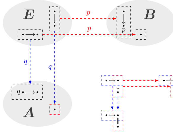
FIGURE 1. The cartesian-vertical factorization of a morphism in a span: a fibration determines a factorization system on E in the sense that every f : e \rightarrow e' in E admits a factorization as a p -vertical arrow followed by a p -cartesian arrow; dually, an opfibration determines a q -vertical, q -cocartesian factorization.
