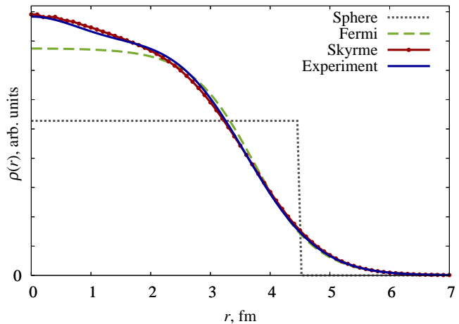
Figure 1. (colors online) Comparison between an experimental (“Gauss”) and different model charge distributions for ^{40}\text{Ca} nucleus. The names of the distributions are explained in Section II A.
