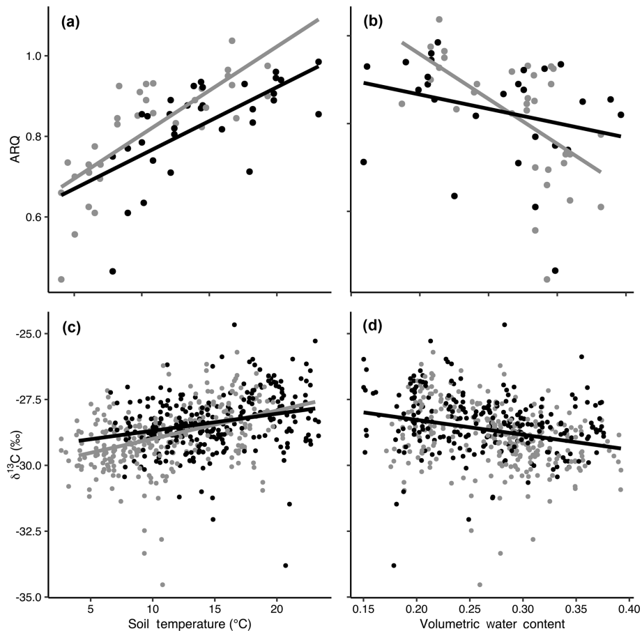
Figure 3. The relationships of apparent respiration quotient (ARQ) by soil temperature ( a ; n = 65 ) and soil moisture ( b ; n = 60 ) and \delta^{13}\text{C}_2 by soil temperature ( c ; n = 565 ) and soil moisture ( d ; n = 535 ). Gray and black points represent data from control and heated gas wells, respectively. The lines show the fit of a mixed-model regression between each variable, where individual gas well was treated as a random effect. Separate grey (control) and black (heated) lines indicate that there was a significant effect of warming treatment on the relationship between the response variable and soil temperature or volumetric water content.
