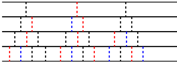
FIGURE 19. An example of F_\tau with edges shown in blue with the minimal state \tau shown as red edges.
