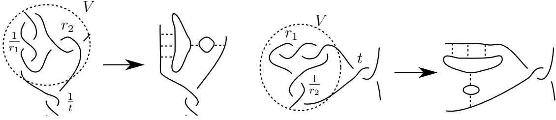
FIGURE 28. Examples of applying the all-B state to V and the resulting disjoint circles for moves sending tangles \frac{1}{t} to (\frac{1}{r_1} \oplus r_2) * \frac{1}{t} and sending t to (r_1 * \frac{1}{r_2}) \oplus t . The tangles that form part of V are encircled.
