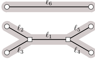
FIGURE 4. A separatrix diagram for \mathcal{Q}(1^2, -1^6)
