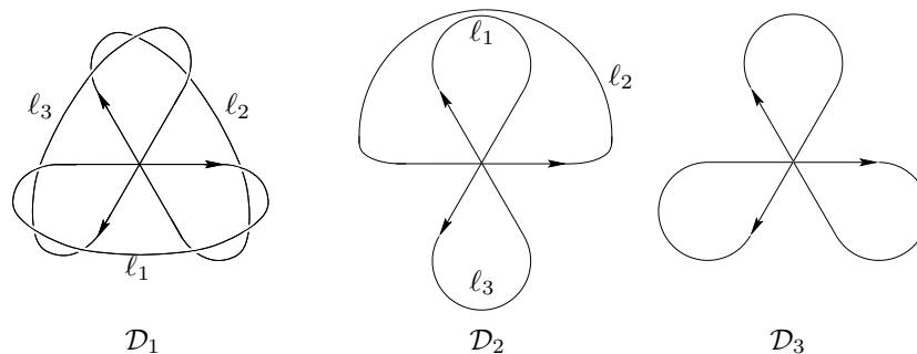
FIGURE 1. The separatrix diagrams represent from left to right a square-tiled surface glued from: \mathcal{D}_1 — one cylinder; \mathcal{D}_2 — two cylinders; \mathcal{D}_3 — not realizable by a square-tiled surface.
