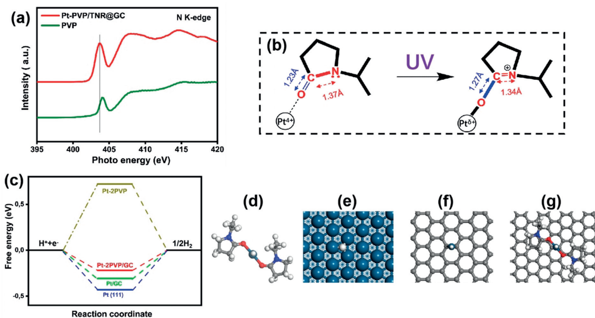
Figure 4. a) N K-edge XANES spectra of PVP and Pt-PVP/TNR@GC. b) Change in the local structure of a Pt atom coordinated by PVP before and after UV irradiation; bond lengths were obtained from DFT calculations, see Table S3 in the Supporting Information for details. c) Free energy diagram of hydrogen evolution at zero potential and pH 0 for Pt-2PVP/GC, Pt-2PVP, Pt/GC, and Pt(111). d-g) The optimized structures of PVP coordinated to Pt atoms in the gas phase (Pt-2PVP) and in Pt(111), (Pt/GC), and Pt-2PVP supported on graphitic carbon (Pt-2PVP/GC) with adsorbed H, respectively. White, gray, blue, red, and cyan balls represent H, C, N, O, and Pt atoms, respectively. Graphitic carbon is modeled by graphene in the DFT calculations.
