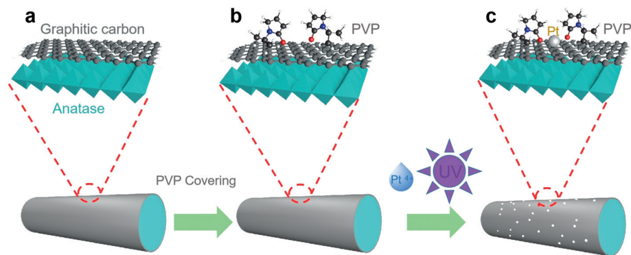
Scheme 1. Illustration of the synthesis of Pt-PVP/TNR@GC catalysts.
