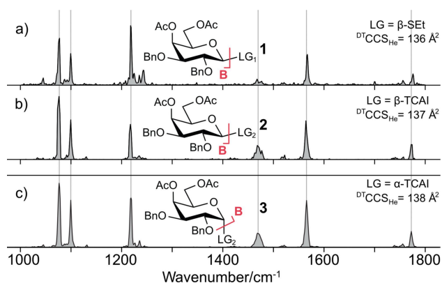
Figure 1. Impact of the leaving group on the structure of B-type ions. Infrared spectra of glycosyl cations generated from a) β-thioethyl (1, SEt), b) β-trichloroacetimidate (2, TCAI) and c) α-trichloroacetimidate (3, TCAI) precursors of 4,6-di- O -acetyl-2,3-di- O -benzyl- D -galactopyranoside. Regardless of the chemical type and anomericity of the leaving group, similar IR signatures are obtained. Ac: acetyl; Bn: benzyl; LG: leaving group, DT CCS He : Drift-tube collision cross section in He.
