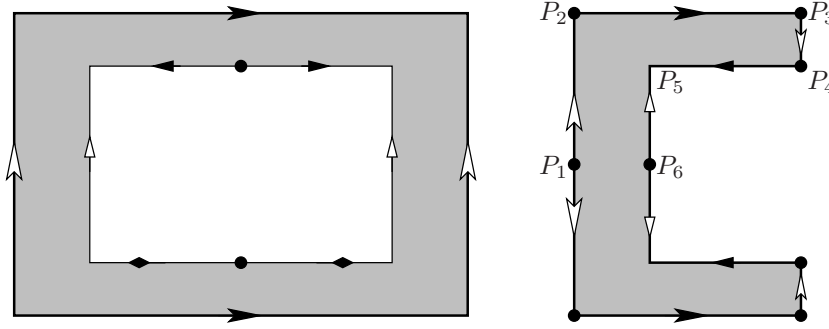
FIGURE 6. A surface \tilde{S} in the hyperelliptic locus \mathcal{Q}^{hyp}(1^2, -1^2) (on the left) is a double cover over the underlying surface S in \mathcal{Q}(1, -1^5) (on the right) ramified at four simple poles represented by bold dots.
