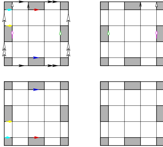
FIGURE 11. The translation surface X \in \mathcal{H}(2^{12}) obtained as the quotient over \mathbb{Z} \oplus \mathbb{Z} of an unfolded wind-tree billiard table in the left picture in Figure 10.
