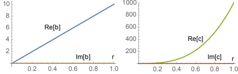
Figure 7. The geometry of the Euclidean saddle point on the positive imaginary axis. Both b(r) and c(r) are real valued. At the origin b has a small negative value and then passes through zero to reach the final value b(1) = 10 . Here we used the same parameter values as in Fig. 6.
