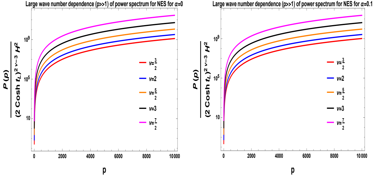
(a) Large wave number dependence of NES power spectrum for \alpha = 0 . (b) Large wave number dependence of NES power spectrum for \alpha = 0.1 .
