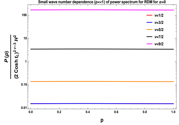
(b) Small wave number dependence of RDM power spectrum for \alpha = 0 and \nu = 1/2, 3/2, 5/2, 7/2, 9/2 .
