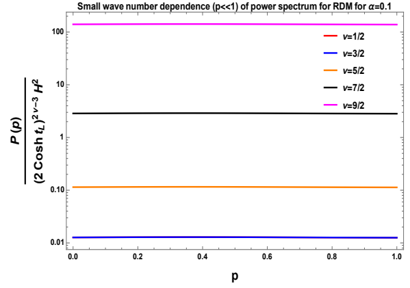
(d) Small wave number dependence of RDM power spectrum for \alpha = 0.1 and \nu = 1/2, 3/2, 5/2, 7/2, 9/2 .
