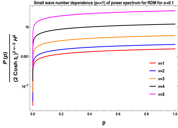
(c) Small wave number dependence of RDM power spectrum for \alpha = 0.1 and \nu = 1, 2, 3, 4, 5 .
