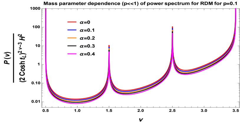
(e) Mass parameter dependence of RDM power spectrum in p \ll 1 .
