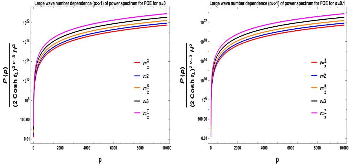
(a) Large wave number dependence of FOE power spectrum for \alpha = 0 . (b) Large wave number dependence of FOE power spectrum for \alpha = 0.1 .
