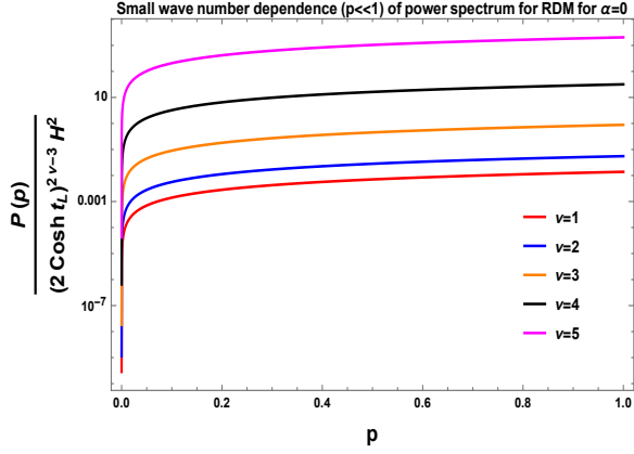
(a) Small wave number dependence of RDM power spectrum for \alpha = 0 and \nu = 1, 2, 3, 4, 5 .
