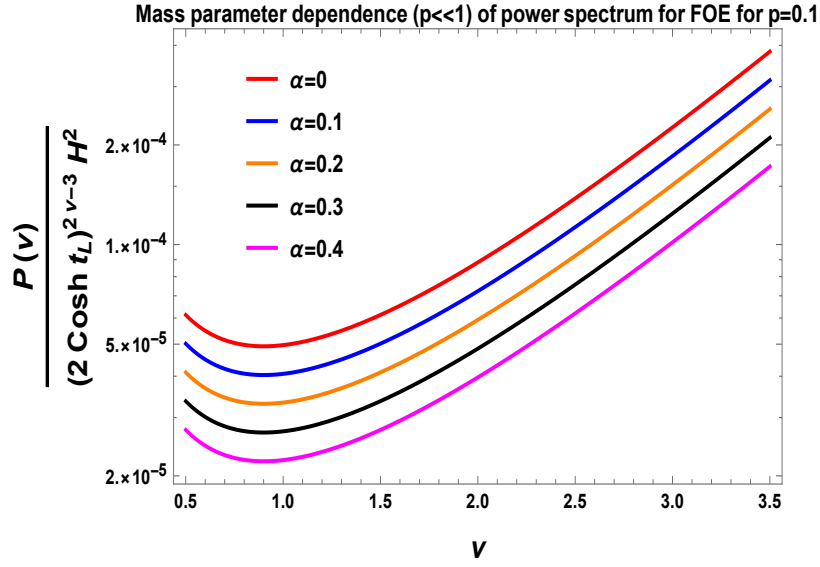
(c) Mass parameter dependence of FOE power spectrum for p \ll 1 .
