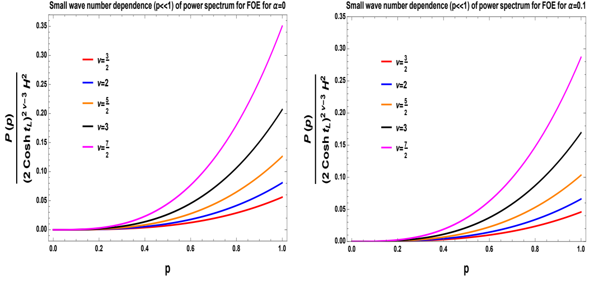
(a) Small wave number dependence of FOE power spectrum for \alpha = 0 . (b) Small wave number dependence of FOE power spectrum for \alpha = 0.1 .
