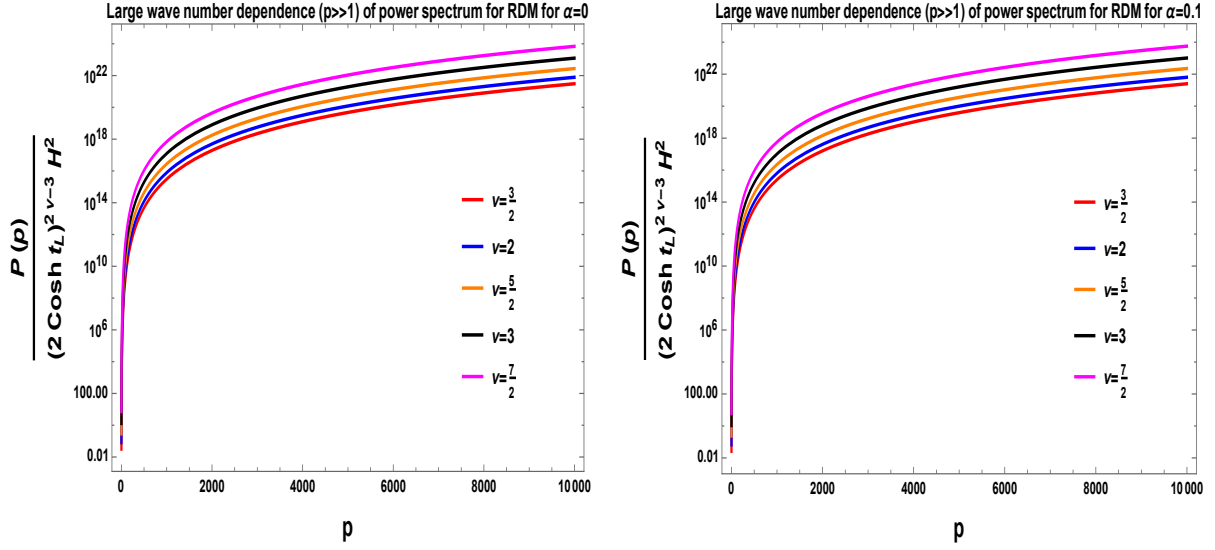
(a) Large wave number dependence of RDM power spectrum for \alpha = 0 . (b) Large wave number dependence of RDM power spectrum for \alpha = 0.1 .
