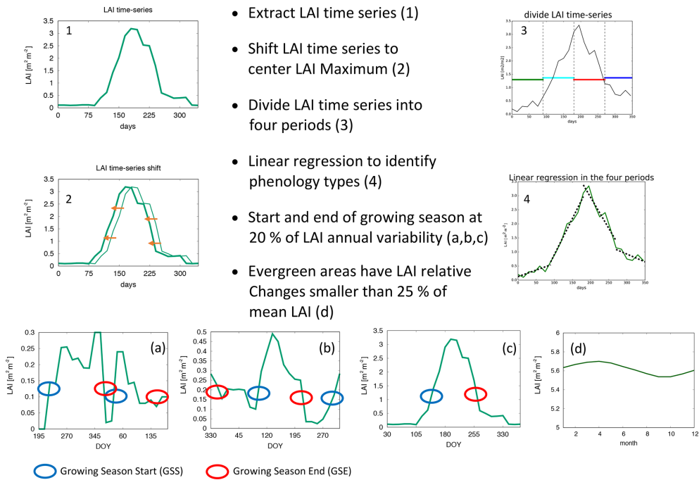
Figure 1. Scheme of the four growing season types method used in evaluating the start and end of the growing season.
