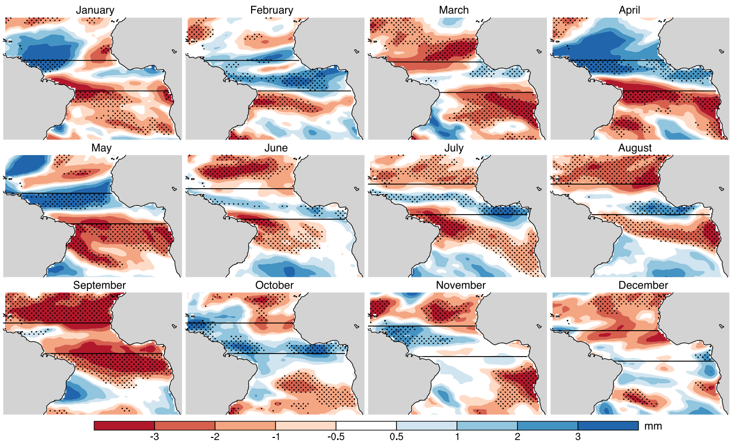
Figure 3. Monthly mean composite difference in water vapor path (shading) between the 5 years with the largest and the 5 years with the smallest \mathcal{N}_{\text{long}} . The black horizontal lines enclose the ITCZ region, as averaged over the 10 considered years. Stippling indicates significance at the 90% level, computed by randomly drawing two sets of 5 years each, computing the difference between the two sets, repeating this 30 times, and stippling the points where, in the subtropics (ITCZ region), the composite difference shows a stronger drying (moistening) at the 90% level.
