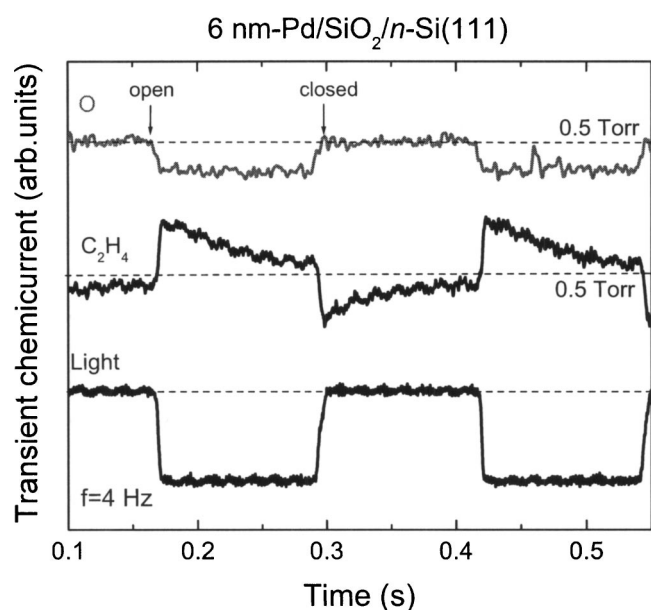
FIG. 2. Time-averaged single pulse currents recorded at Pd-MOS diodes during exposure to O, C_2H_4 and white light. The signals were modulated at 4 Hz and the dashed lines indicate the signal base line. The gas pressure of 0.5 Torr in the first beam chamber is a relative measure of the gas particle flux.
