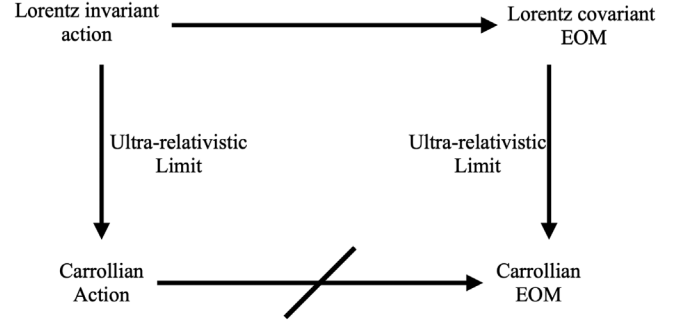
FIG. 2. The process of taking Carrollian (ultrarelativistic) limit and applying variational derivative on action functional does not commute.
