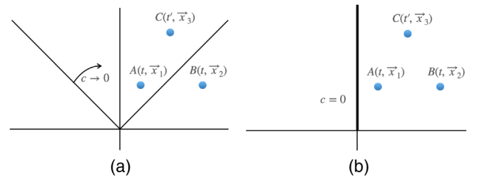
FIG. 1. In the panel (a) above, the points A and C are causally connected, whereas the interval A - B is acausal, in Minkowski space. To get Carroll space-time as the c \rightarrow 0 limit, one should collapse the light cone to a single line, as in panel (b). In Carroll space-time, none of the points A, B , and C are causally connected, unless the events take place exactly at the same spatial points.
