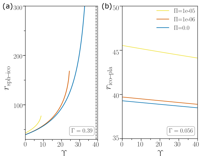
Fig. 3. Critical size for the faceting (a) and flattening (b) transitions, obtained by solving the equations \mathcal{E}_{\text{sph}} = \mathcal{E}_{\text{ico}} and \mathcal{E}_{\text{ico}} = \mathcal{E}_{\text{pla}} with respect to r , versus the \Upsilon parameter. Note in (a) that for each \Pi , there is a maximal \Upsilon beyond which no critical radius exist for this transition, as all droplets are icosahedral.
