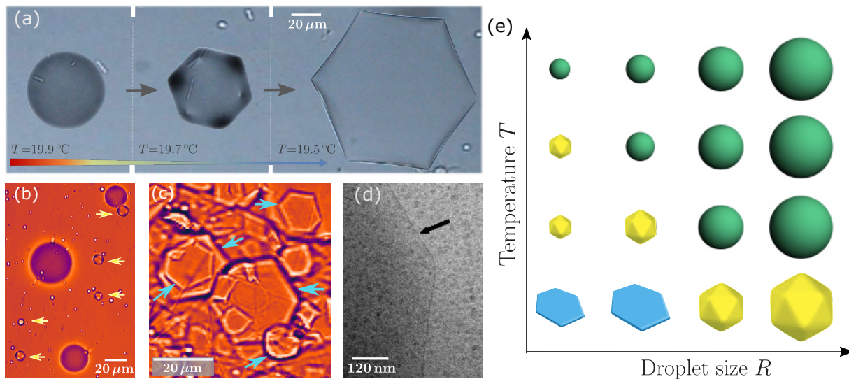
Fig. 1. Experimental images of the faceting of spherical droplets and flattening of icosahedra. (a) Light microscopy snapshots of the volume-conserving faceting and flattening of a single spherical droplet of radius R \sim 25 \mu\text{m} as temperature is lowered. (b) Typical configuration of a polydispersed sample showing large spherical and small icosahedral droplets (highlighted by arrows). (c) Icosahedral droplets and platelets are oriented with a flat face orthogonal to the direction of gravity. (d) CryoTEM image of the interface of an icosahedral droplet, revealing that the thickness of the crystalline structure is close to 3 nm, corresponding solely to the interfacially-frozen monolayer (reproduced and modified with permission from [9]). (e) Schematic of the phase diagram of the droplets based on the experimental observations, with the triangulated surfaces used in the numerical calculations of the energy [see Eq. (3)].
