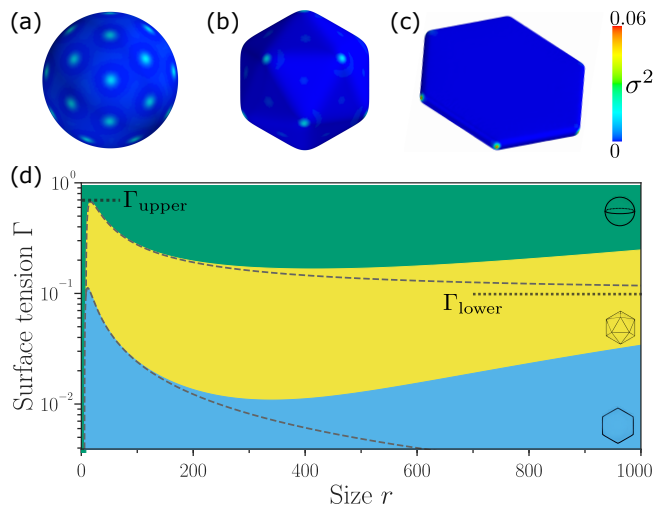
Fig. 2. (a-c) Defect-induced stress field \sigma^2 on the crystalline interface with screening dislocations, computed from the charge density \eta in Eq. (5). (d) Morphological phase diagram in the (r, \Gamma) -plane obtained from a comparison of the energies of spherical, icosahedral and platelet-shaped droplets calculated via Eq. (3). The bound values of \Gamma for faceting, Eq. (6), are indicated with dotted lines. The dashed lines correspond to the phase boundaries when buoyancy effects are ignored. To create this diagram we chose \Upsilon = 10 and \Pi = 10^{-7} .
