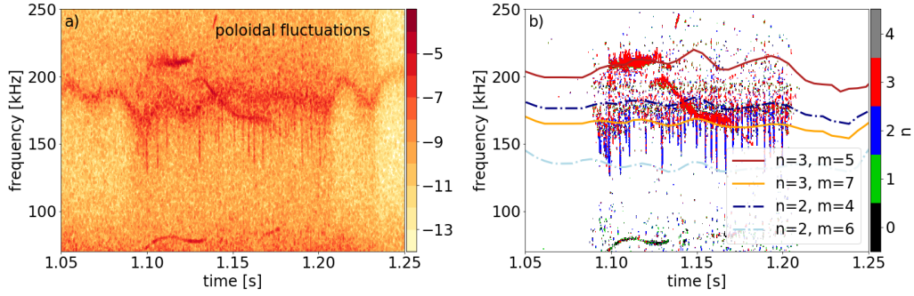
Figure 5: a) Zoom of the magnetic spectrogram shown in figure 4b. b) Toroidal mode number analysis together with the expected frequencies of n=3 and n=2 TAEs with different poloidal mode numbers.
