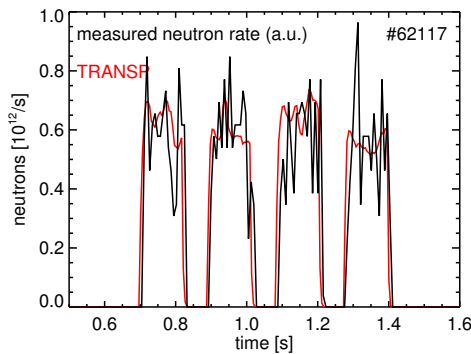
Figure 12: Measured neutron rates compared to a neoclassical TRANSP simulation (red).
