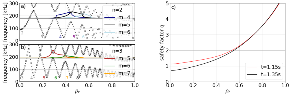
Figure 6: Predicted Alfvén continuum (black crosses) of n=2 (a) and n=3 (b) modes at t=1.15 s. c) Safety factor profiles for two different time points with and without ECRH.
