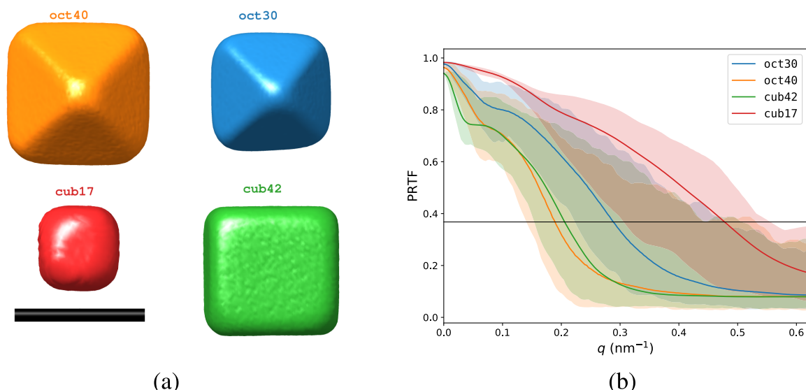
Fig. 5. Phase retrieval. (a) Isosurface plots of electron densities recovered after phase retrieval (scale bar is 40 nm). The asymmetric structures of the octahedra are clearly evident (see Visualization 2 and Fig. S7). (b) Smoothed phase retrieval transfer function (PRTF) measuring reproducibility of phases as a function of q . The solid lines represent the azimuthal average PRTF conventionally used to determine the resolution of the structure. The shaded region around each line indicates the range of values at each q . The typical 1/e cutoff is shown in black.
