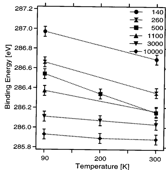
FIG. 3. The temperature-dependent CO C 1s binding energy shifts below the dissociation and desorption thresholds for the different island sizes.
