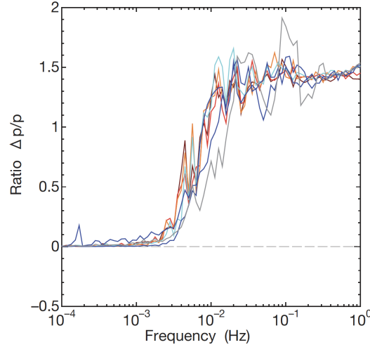
Fig. 13 Relative differences in air pressure between the front and end chambers. Both air pressures are almost identical (within 10 % difference) below \sim 3 mHz and they are uncorrelated above \sim 10 mHz. Different datasets are shown in different colors to see the repeatability and the fluctuation.
