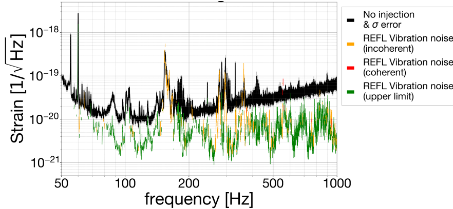
Fig. 7 Result of an acoustic-injection test performed during FPMI commissioning in December 2019 [53]. Strain sensitivity without PEM injection (black), with projected acoustic noise (orange, incoherent; red, coherent), and the 3\sigma upper limit to the acoustic noise (green).
