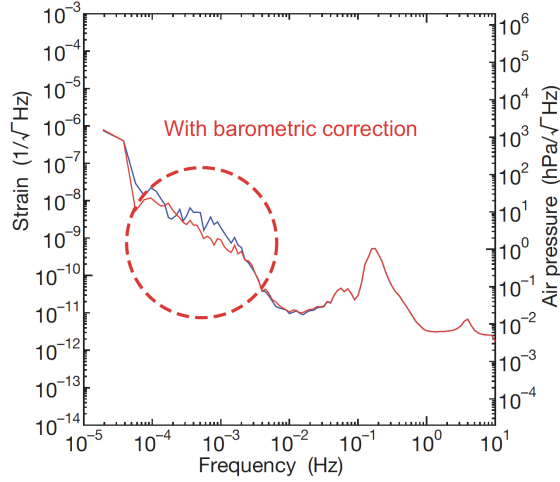
Fig. 14 Ground-strain spectra before (blue) and after (red) correction using the measured air pressure. The background strain is reduced by \sim 1/3 at best in the 10^{-4} – 10^{-3} -Hz region (within the dashed red circle). This limited reduction suggests that the background strain is not determined simply by the local air pressure but also is affected by the regional air pressures which may have different correlations to the local air pressure.
