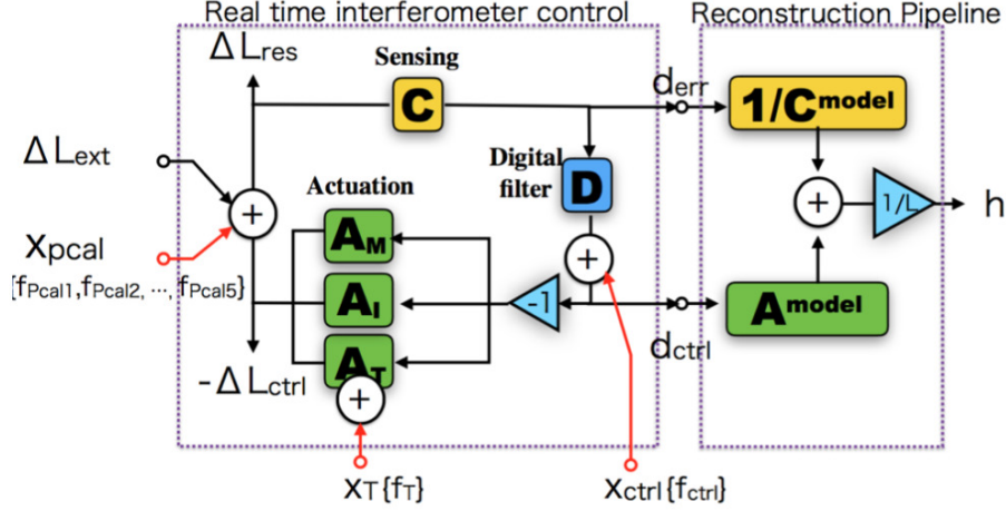
Fig. 1 Diagram of the DARM control loop and the reconstruction pipeline. The DARM model consists of actuation and sensing parts. The actuator part corresponds to the transfer function from a digital-to-analog converter (DAC) to the displacement of the mirror. The sensing part is a combination of interferometer and photo-detector responses. The quantities d_{err} and d_{ctrl} are error and control signals, which are outputs from the interferometer. Using this DARM model, we can construct actuator part and sensing part for reconstructing the signal. Red arrows show injections from outside the feedback loop.
