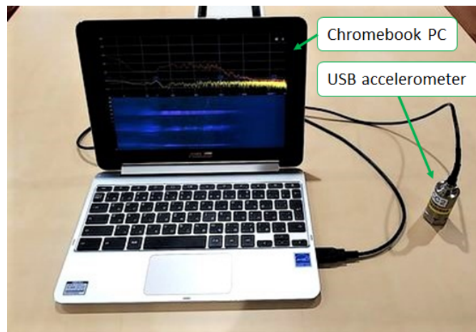
Fig. 6 Photograph of a Chromebook with a USB accelerometer. The real-time spectrum and a spectrogram generated by free software are displayed.
