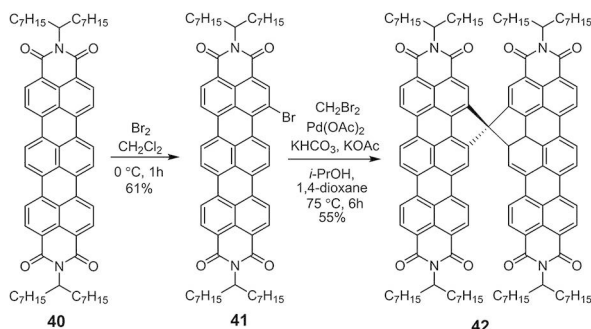
Scheme 16. Synthesis of spiro-fused terrylene diimide compound 42 .
