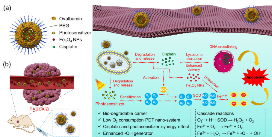
Scheme 1. Illustration of a) the structure of the OVA-NCs containing photosensitizer, Fe 3 O 4 NPs, and cisplatin. b) Targeted delivery of the OVA-NCs in the hypoxia tumor site via EPR effect. c) The mechanism of the PDT/chemotherapy combination therapy with integrated tandem Fenton reactions in the intracellular environment.
