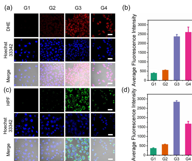
Figure 4. a) Detection of \text{O}_2^{\cdot-} ( \lambda_{\text{ex}}=488 \text{ nm} , \lambda_{\text{em}}=590\text{--}610 \text{ nm} ) and c) \cdot\text{OH} ( \lambda_{\text{ex}}=488 \text{ nm} , \lambda_{\text{em}}=500\text{--}550 \text{ nm} ) generated in MCF-7 cells under hypoxia with different nanocapsule treatments by using CLSM. The fluorescence of Hoechst 33342 was excited at 405 nm and collected at 420–480 nm. Scale bar = 40 \mu\text{m} . b) The quantitative analysis of fluorescence intensity of DHE for the detection of \text{O}_2^{\cdot-} . d) The quantitative analysis of fluorescence intensity of HPF for the detection of \cdot\text{OH} . Key: control (G1), FePtNBS@OVA (G2), FePtNBS@OVA + Light (G3), FePtNBS@OVA + DFOA + Light (G4). Light irradiation was carried out by 660 nm LED light ( 35 \text{ mWcm}^{-2} , 4 min, 8.4 \text{ J cm}^{-2} ). Data are given as the mean \pm SD ( n=3 ).
