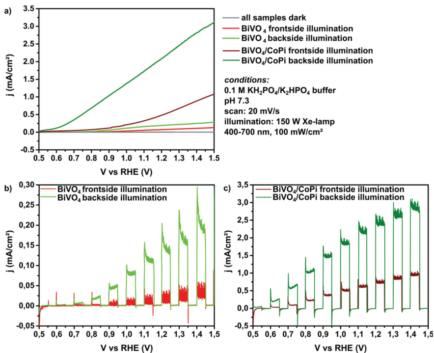
Fig. 11: (a) j - V curves of \text{BiVO}_4 thin films with and without a layer of CoPi water oxidation catalyst under continuous illumination, j - V curves of \text{BiVO}_4 thin films (b) without and (c) with a layer of CoPi water oxidation catalyst under chopped illumination.
