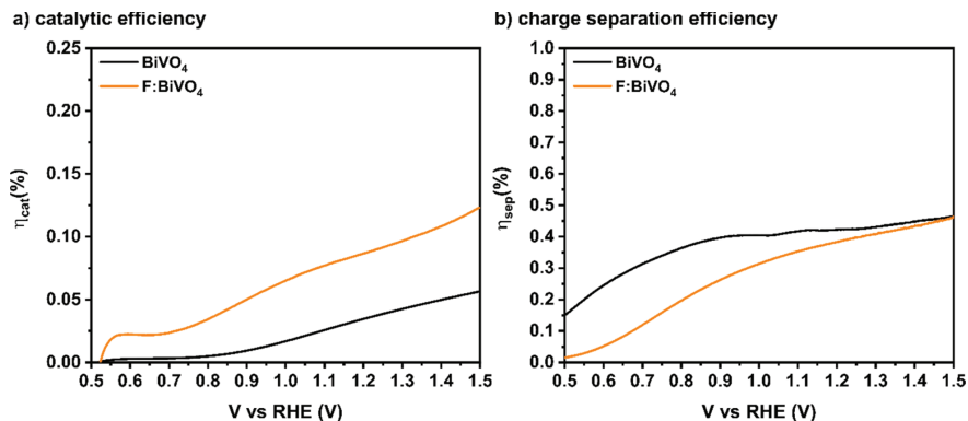
Fig. 16: (a) Catalytic efficiency and (b) charge separation efficiency for BiVO 4 and F:BiVO 4 thin film photoanodes. Backside illumination was used for recording photocurrents for water oxidation and sulfite oxidation. Adapted with permission from ref. [25]. Copyright 2019 American Chemical Society.
