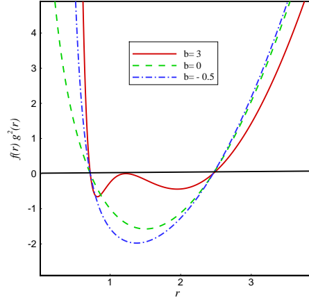
Figure 2. The behavior of -\mathbf{g}_{tt} = f(r)g^2(r) for charged mimetic black holes in 3D and different b . Here we have taken M = 2 , l = 1 , q = 1.5 .
