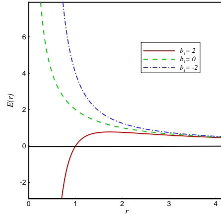
Figure 3. The behavior of the electric field F_{tr} = E(r) for 3D charged mimetic black holes with q = 2 .
