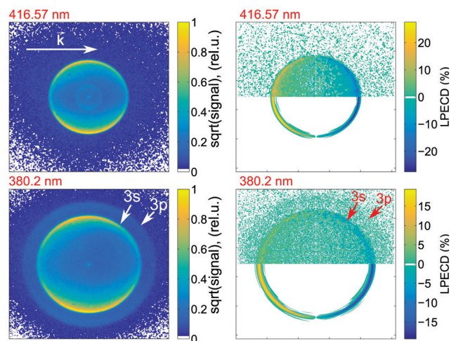
Fig. 4 Photoelectron velocity map images for (S)-(+)-fenchone ionized via 2 + 1 REMPI via the 0_0^0 transition to the 3s state using 416.57 nm light (top row) and via transitions to both the 3s and 3p states using 380.2 nm light (bottom row). The left-hand column shows the photoelectron images obtained using LIN and the right-hand column shows the antisymmetrized PECD images. In the upper half of each PECD image, the raw data is shown and in the lower half the Abel-inverted image is shown. In the images obtained with 380.2 nm light, the kinetic energy of the intense inner ring and weak outer ring correspond to vertical ionization from the 3s and 3p Rydberg states, respectively. The white vector shows the direction of the excitation laser beam.
