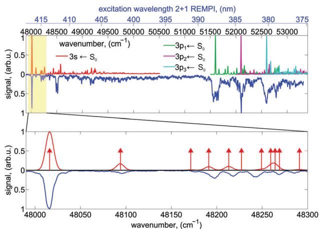
Fig. 2 The experimental 2 + 1 REMPI spectrum of the 3s \leftarrow n and 3p \leftarrow n transitions of fenphone recorded with linearly polarized light is shown in blue. For comparison, the calculated Franck–Condon profiles for the transition to the 3s state (red) and the transitions to the three components of the 3p state, denoted here by 3p_1 , 3p_2 , and 3p_3 (green, purple, turquoise) are shown. The origin of the individual profiles have been shifted by about 4500 \text{ cm}^{-1} (namely 4348 \text{ cm}^{-1} , 4257 \text{ cm}^{-1} , 4466 \text{ cm}^{-1} , 4746 \text{ cm}^{-1} for 3s , 3p_1 , 3p_2 , 3p_3 , respectively) to higher wavenumbers compared to the computed 0–0 transition wavenumbers. See text for more information. Intensities of the different FC profiles were scaled such that all 0–0 transitions are normalized to the same intensity. In the bottom panel, an enlarged view of the region around the band origin of the 3s state, where the vibrational levels are well resolved, is shown. Transitions to individual vibrational eigenstates are indicated by red arrows with their length being unrelated to the Franck–Condon factor.
