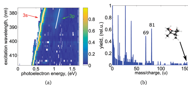
Fig. 3 (a) Wavelength-dependent PES derived from the LIN PADs for ( S )-(+)fenchone after Abel-inversion using polar onion peeling. 64 Every row represents a single measurement, where up to two distinct electronic intermediates were observed. The expected energy scaling with \hbar\omega is indicated by the white lines. (b) Mass spectrum for ( S )-(+)fenchone obtained at the 3s band origin at 416.57 nm. A detailed discussion can be found in the text.
