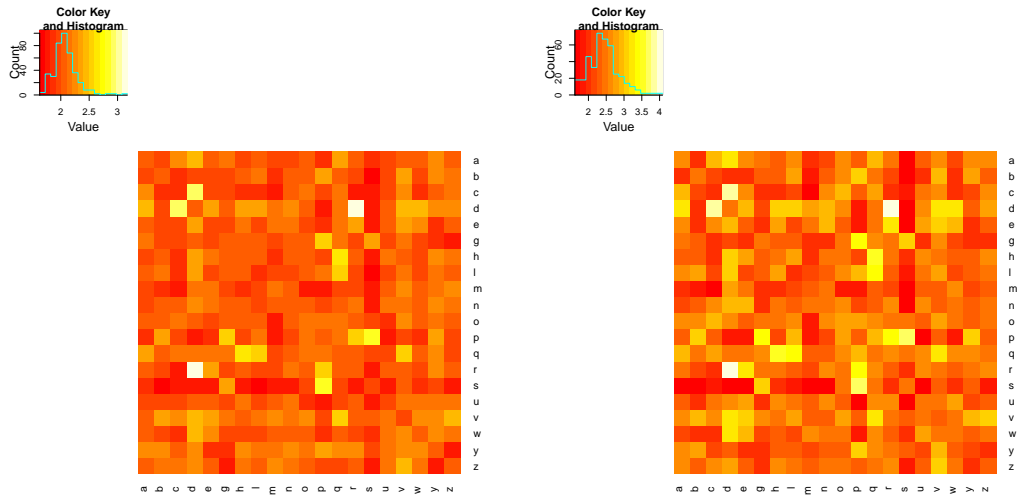
■ Figure 7 Log of mean value computation time in ms for LMF (left) and Binary Search (right).
