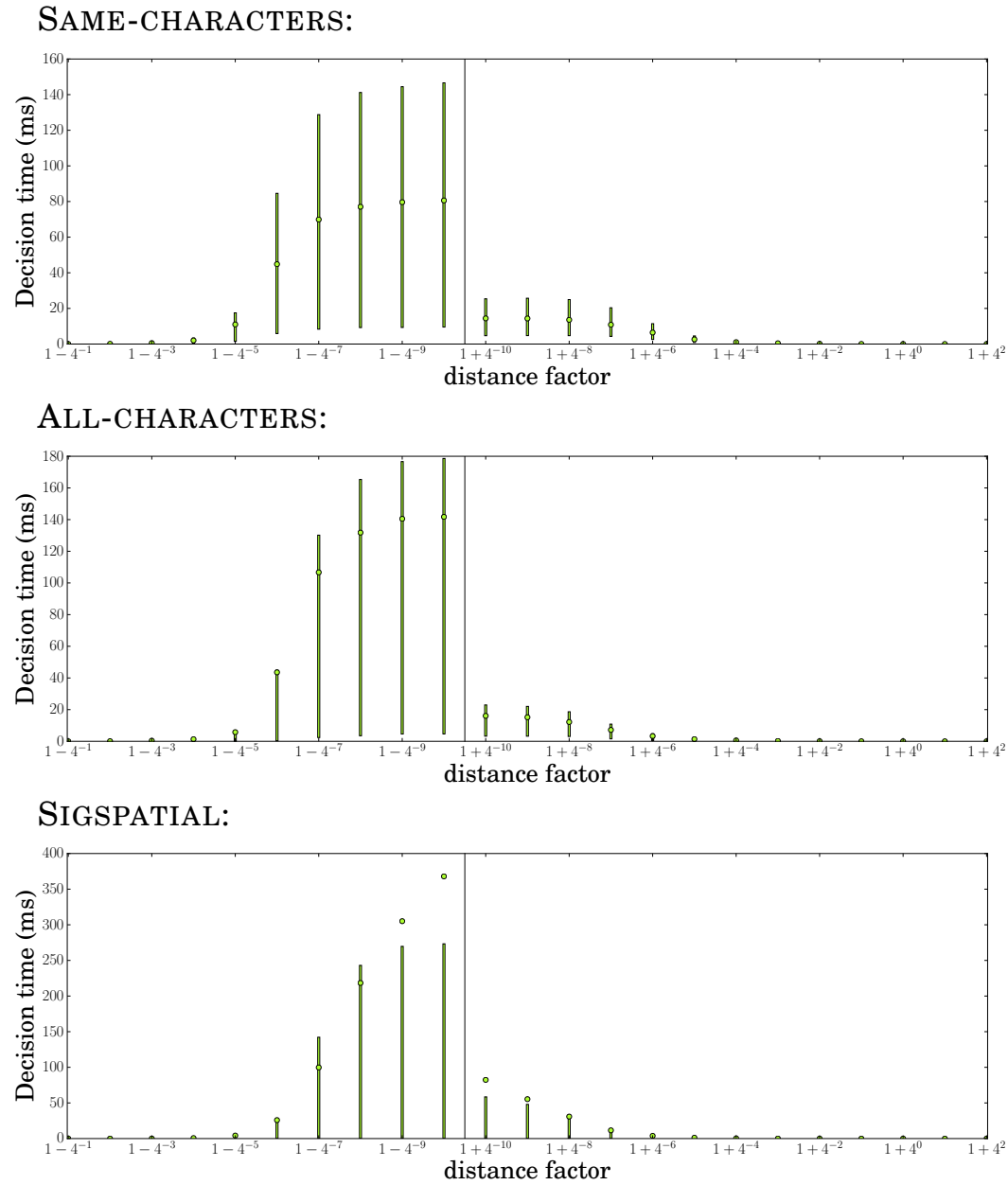
■ Figure 4 Running time for our decider. We plot the mean running times over 1000 NO (or YES) queries with a test distance of approximately (1 - 4^{-\ell}) (or (1 + 4^{-\ell}) ) times the true Fréchet distance under translation, as well as the interval between the lower and upper quartile over the queries.
