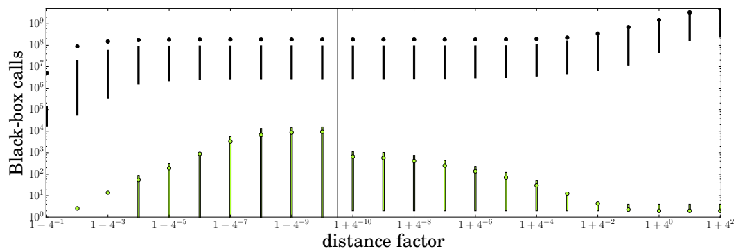
■ Figure 5 Number of black-box calls to the fixed-translation Fréchet decoder made by our decoder (below, in green), as well as an estimate of the arrangement complexity, i.e., number of calls of a naive algorithm (above, in black). We plot the mean number of calls and arrangement complexity over 1000 NO (or YES) queries with a test distance of approximately (1 - 4^{-\ell}) (or (1 + 4^{-\ell}) ) times the true Fréchet distance under translation, as well as the interval between the lower and upper quartile over the queries.
