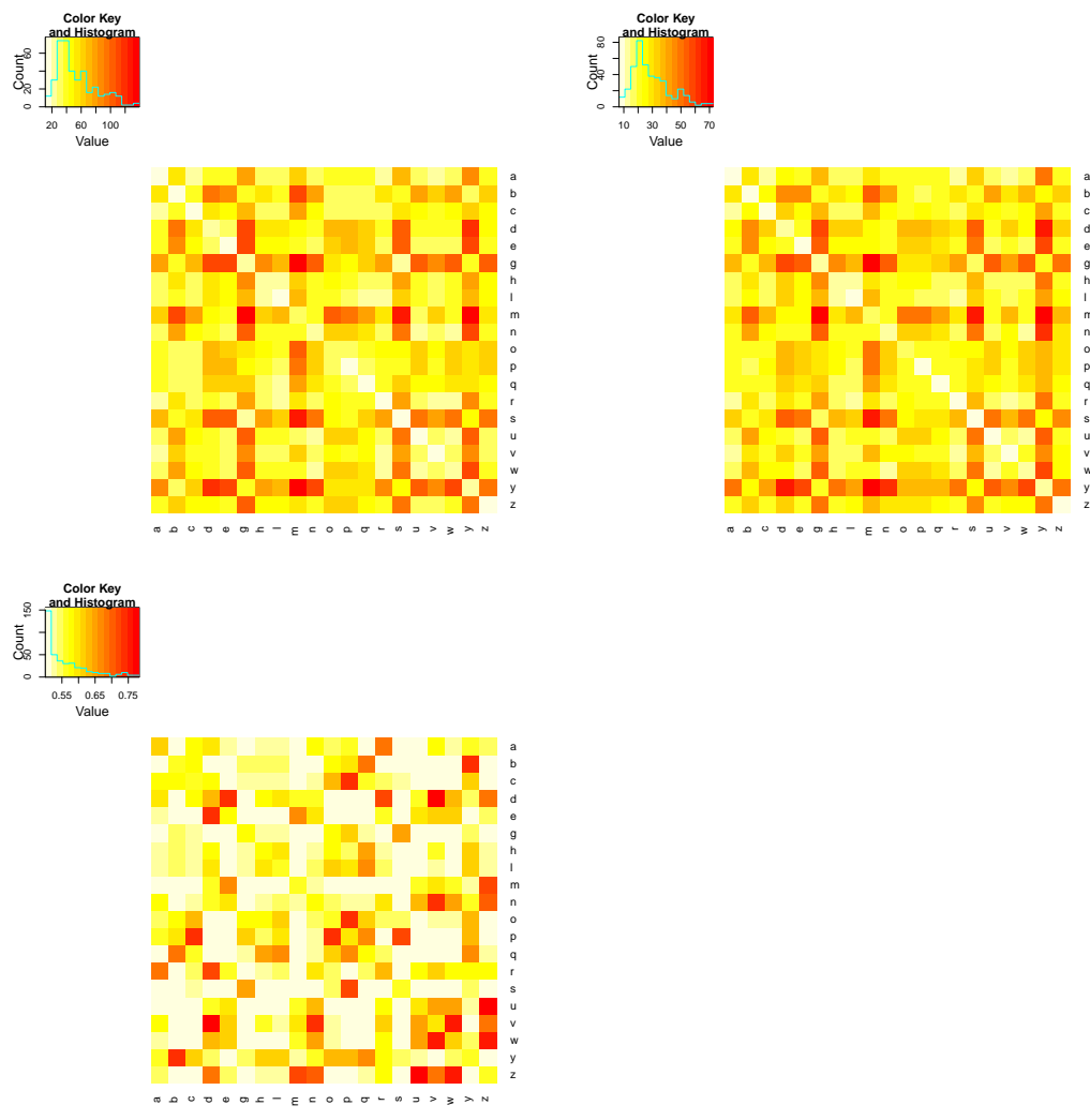
Figure 9 Average Fréchet distance value (top left) and average Fréchet distance under translation value (top right), as well as the quotient of these values (bottom left).
