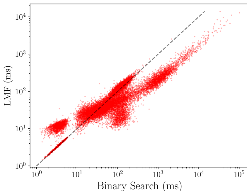
■ Figure 6 Running times of LMF and binary search on set of randomly sampled CHARACTERS curves.
