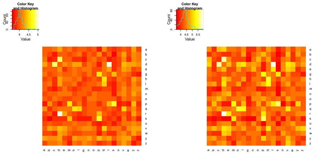
■ Figure 8 Log of mean number of black-box calls for LMF (left) and Binary Search (right).
