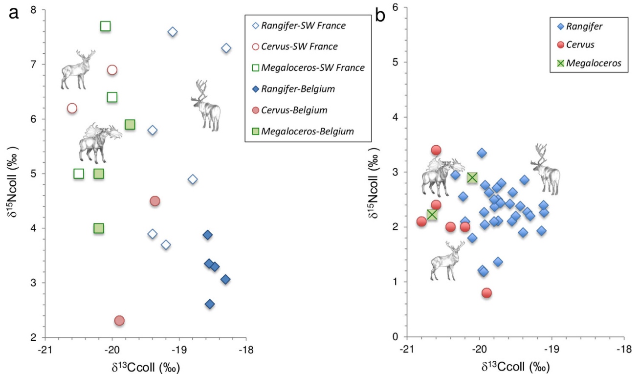
Figure 4. (a) Stable isotope values of reindeer ( Rangifer ), red deer ( Cervus ) and Megaloceros before the LGM in SW France and Belgium and (b) after the LGM in the Swabian, Swiss and French Jura indicate a decrease in the distinction between the isotope signatures of the three cervid species after the LGM, which might be due to overlapping diet and habitat. The deer drawings were kindly prepared and provided by Kerttu Majander.
