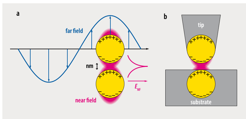
FIGURE 1: A localized surface plasmon excitation in a nanoparticle dimer (a, yellow) is separated by a few nanometers. The incoming light (blue) stimulates collective oscillations of electrons in the nanoparticles generating a highly localized and intense electromagnetic field (pink) in the gap. A scanning tunneling microscope junction might generate a localized surface plasmon (b). This nano-light is spatially controlled by scanning the plasmonic tip.
