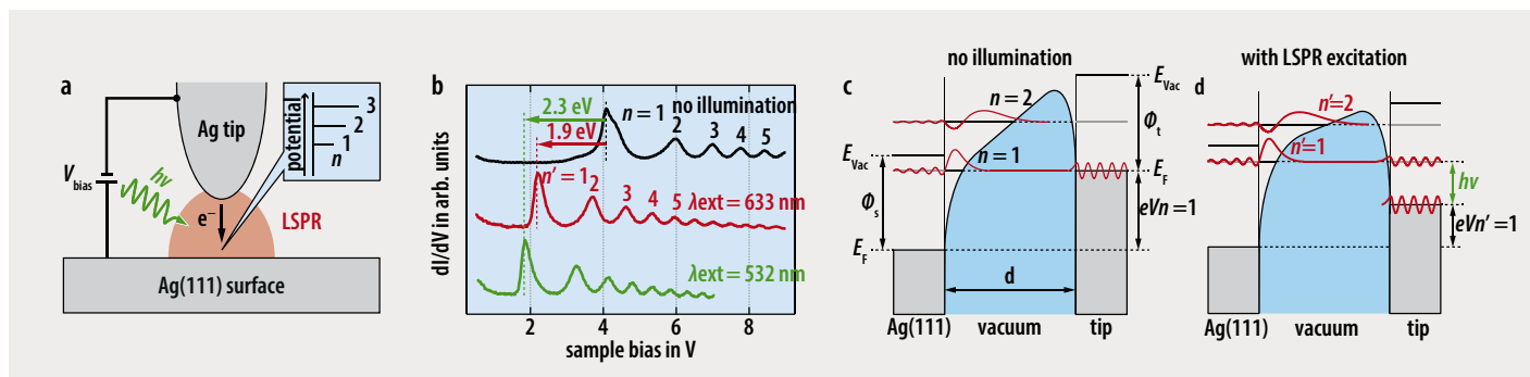
FIGURE 3: Plasmon-assisted resonant electron tunneling is examined in the junction of the Ag tip and the Ag(111) surface (a). The field emission resonance spectra change with and without illumination and depend on the wavelength \lambda_{\text{ext}} (b). The variations stem from the corresponding potential in the junction (blue area in c, d) and the different incident photon energy ( E_F : Fermi level, E_{\text{vac}} : vacuum level, \Phi_{s(t)} : work function of surface (tip), d : gap distance, n(n') : index of the resonances, V_{n(n')} : voltage of the resonances, h\nu : incident photon energy).
