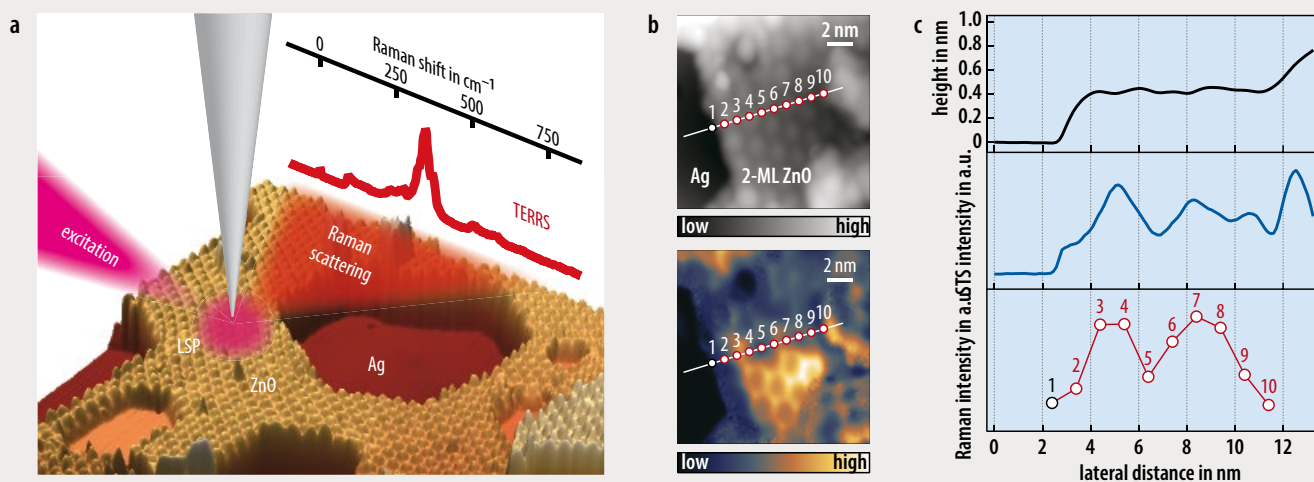
FIGURE 5: The localized surface plasmon is excited at the apex of a sharp tip which generates a locally enhanced Raman scattering signal from ultrathin zinc oxide films epitaxially grown on a Ag(111) surface (a). A scanning tunneling microscope image (b, top) and a scanning tunneling spectroscopy mapping (bottom) show the boundary between the Ag surface and the ultrathin zinc oxide film. Height and intensities are measured at ten points using scanning tunneling microscopy (c, black), scanning tunneling spectroscopy (blue) and tip-enhanced resonance Raman spectroscopy (red).
