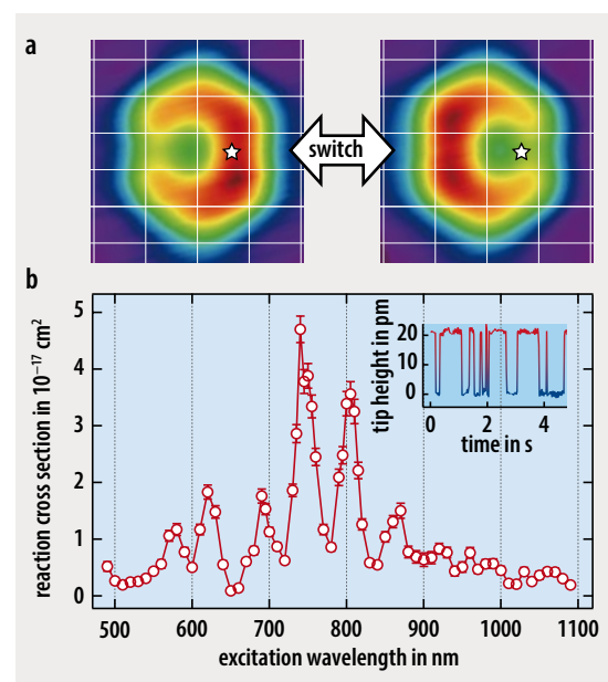
FIGURE 4: Scanning tunneling microscope images prove the single-molecule tautomerization of porphycene (a). The near-field action spectrum obtained by the Au tip with a groove on the shaft (b) shows a modulation. The two-state random telegraph noise results from plasmon-driven single-molecule tautomerization (inset).
