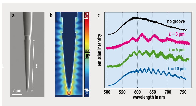
FIGURE 2: Focused ion-beam milling produces Au tips with a single groove on their shafts at a distance L to the apex of the tip (a, scanning electron micrograph). The scanning tunneling luminescence varies due to the plasmonic Fabry-Pérot interference (b, simulation). The emission spectra depend on the distance L between groove and apex (c).
