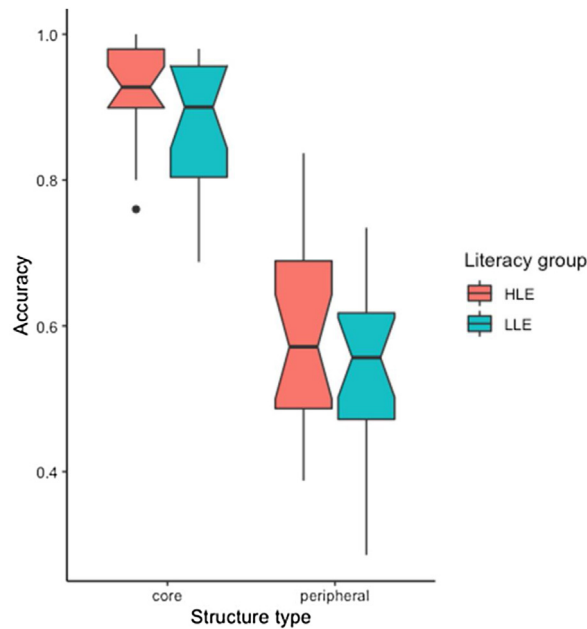
Fig. 3. Notched box-and-whisker plot showing the distribution of participant-level accuracy by literacy group, aggregated by structure type. HLE = High Literacy Experience; LLE = Low Literacy Experience. Each coloured box represents the interquartile range (IQR, i.e., 25th–75th percentile); the ‘notches’ correspond to 95% confidence intervals for the median (marked in black). The ‘whiskers’ extend from minimum to maximum (respectively defined as Q1 - 1.5 \cdot IQR and Q3 + 1.5 \cdot IQR ). The single outlier is shown as a black point.
