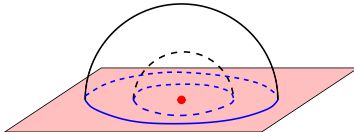
Figure 7. Counting operators on the boundary of half-space \mathbb{R}^2 \times \mathbb{R}_+ leads to combined 2d-3d half-index on S^1 \times D^2 . In radial quantization, the boundary is foliated by concentric circles, which form T^2 boundary of S^1 \times D^2 .
