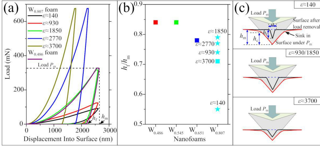
Fig. 4 Nanoindentation of the W_{0.807} foams with various deformation strains and the W_{0.486} nanofoams in the saturated region: (a) representative load-depth curves, (b) ratios between the penetration depth after load removal h_f and maximum penetration depth at peak load h_m , (c) schematic plots of indentation cross-sections (with a sink-in contact profile) made by a Berkovich indenter at the maximum peak load P_m and after load removal.
