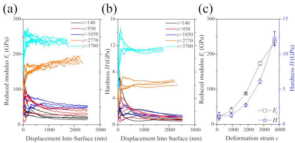
Fig. 7 W_{0.807} foams received from the nanocomposite subjected to various deformation strains: (a) reduced Young's modulus versus displacement curves, (b) hardness versus displacement curves, (c) reduced modulus and hardness values against deformation strains.
