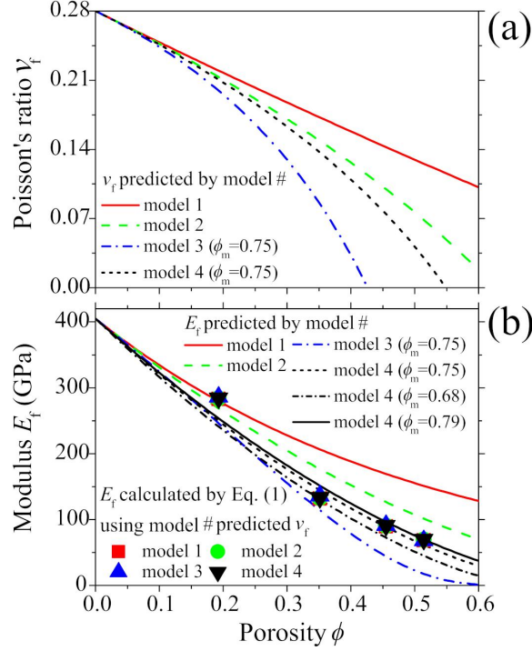
Fig. 6 Effective W nanofoam properties: (a) predicted Poisson's ratio \nu_f versus porosity \phi , (b) Young's modulus E_f versus porosity \phi . A comparison between theoretical model predictions (Table 3) and the experimental data is presented in (b).
