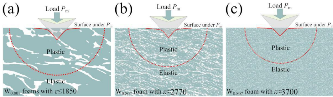
Fig. 10 Schematic drawing of nanoindentation tests on the W_{0.807} foams (blue: W ligaments; white: pores) with: (a) \varepsilon \leq 1850 , corresponding to an elongated and (sub)-micrometer cellular morphology, (b) \varepsilon \approx 2770 , corresponding to an elongated and nanometer cellular morphology, (c) \varepsilon \approx 3700 , corresponding to an equiaxed/spherical and nanometer cellular morphology. A plastic deformation zone beneath the indenter is inside the red dashed line. SEM images of the cross-sections showing the sub-surface microstructures and plastic zones of the W_{0.807} foams with \varepsilon \approx 1850 and \varepsilon \approx 2770 are available in Fig. S7 and 8.
