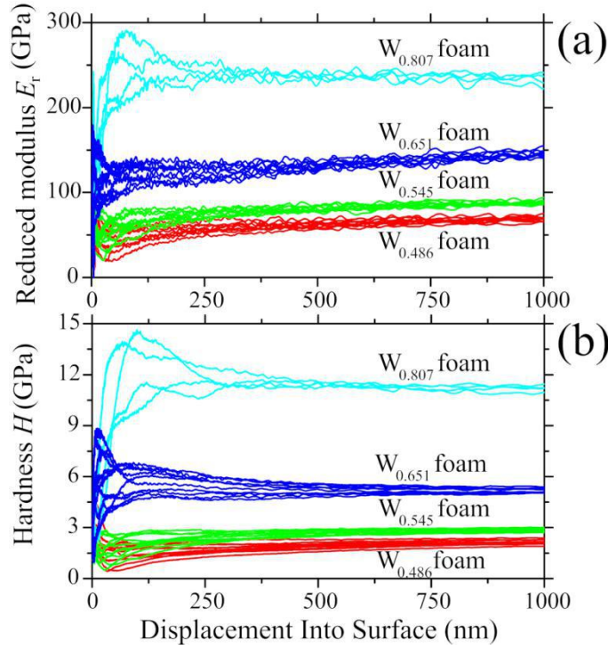
Fig. 5 Nanoindentation data showing (a) the reduced Young's modulus versus displacement curves, and (b) the hardness versus displacement data. For the W_{0.807} nanofoam, experiments were conducted in the region with a deformation strain of about 3700. The nanoindentation for all the other W nanofoams was applied in the saturated regions.
