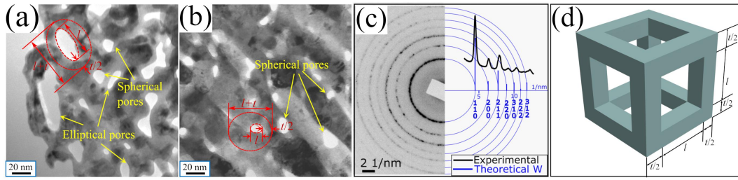
Fig. 2 Bright field TEM images of the (a) W_{0.651} and (b) W_{0.807} nanofoams created from NC W_{80}Cu_{20} in the microstructure saturated region and from NC W_{90}Cu_{10} with \varepsilon \approx 3700 , respectively. Pores in (a) and (b) are shown as bright contrasts while the W grains exhibit dark contrasts. The materials in (a) and (b) have similar SAED patterns given exemplarily in (c). The method to determine the free/unsupported ligament length l and thickness t is illustrated in (d).
