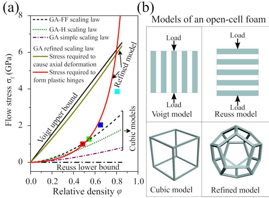
Fig. 9 (a) Relative density dependence of flow strength for the W nanofoams with self-similar and highly ordered cellular structures. The solid squares represent the experimentally calculated strength values. The flow strength predicted by different GA scaling laws and Reuss-Voigt bounds are provided as a comparison. (b) Models applied to obtain different theoretical predictions.
