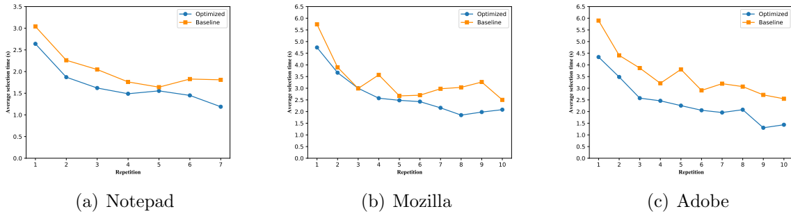
Figure 9: Average selection time per command as a function of number of repetitions
