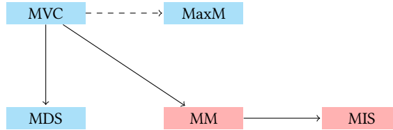
Fig. 5. Relationships between the lower bounds derived for fundamental graph problems (adapted from [22]). Optimization problems marked blue; binary problems marked red. Solid arrows indicate reductions; dashed arrows indicate analogy.
