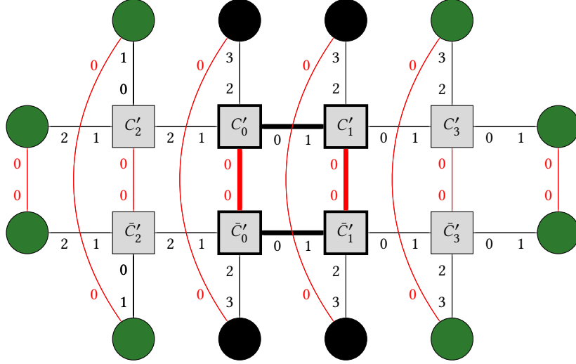
Fig. 6. Construction of H'_2 from G'_2 and \tilde{G}'_2 ; edges corresponding to the perfect matching between nodes in G'_2 and \tilde{G}'_2 are marked red. The edges represented by the thickened lines are 2-hop indistinguishable in H_2 .
