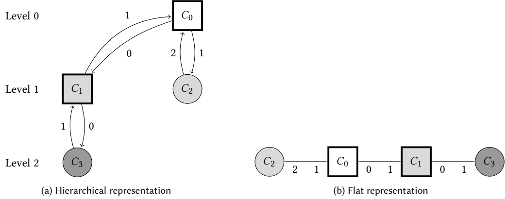
Fig. 1. Representations of CT_1 (shaded by cluster sizes; darker means smaller). Cluster shapes indicate cluster position ( internal or leaf ); core clusters depicted with bold frame. Arc labels are exponents of the parameter \beta , indicating how many neighbors nodes in one cluster have in another.
