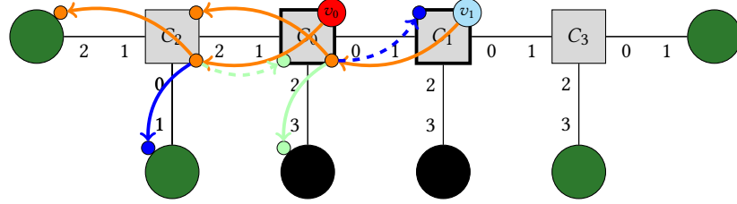
(b) d = 2 from orange nodes at distance d = 1 : because the invariant holds for d = 1 , Corollary 3.17 (p. 9) ensures that Algorithm 1 (p. 8) produces an isomorphism between G_2^2(v_0) and G_2^2(v_1) .
