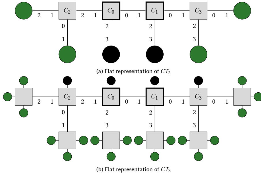
Fig. 2. Representations of CT_2 and CT_3 (colored by cluster types; grey: internal, green: branch consolidation, black: branch instantiation). Cluster shapes correspond to cluster position ( internal or leaf ); core clusters depicted with bold frame. Arc labels are exponents of the parameter \beta , indicating how many neighbors nodes in one cluster have in another.
