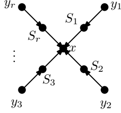
Figure 2: A digraph G in which for every t_i there is a singleton S_i that separates t_i from s but does not separate t_j from s for any j \neq i .
