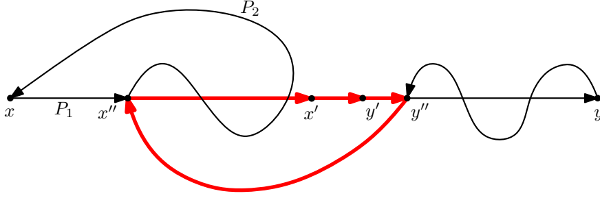
Figure 3: Proof of Lemma 7.
