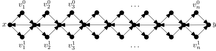
Figure 5: A digraph G with \text{cf}(G) = 3 where every k -representative set of x \rightarrow y -paths has size 2^{\Omega(k)} \log n .
