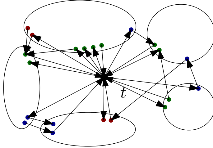
Figure 1: An example for the structure of G - t . The large circles form the strong components C \in \mathcal{C} . The colored dots represent the portals with their color corresponding to their cluster.
