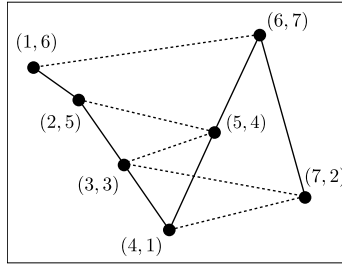
Fig. 1. Permutation \pi = (6, 5, 3, 1, 4, 7, 2) and its incidence graph G_\pi . Solid lines indicate neighbors by index (L-R), dashed lines indicate neighbors by value (U-D). Indices plotted on x -coordinate, values plotted on y -coordinate.
