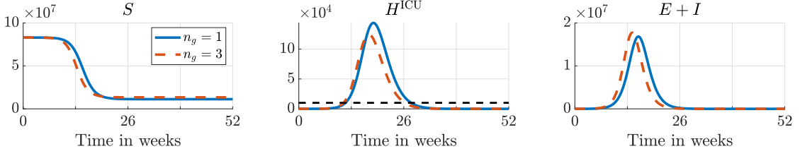
Figure 2: Evolution of the pandemic without countermeasures for one and three age groups over one year; the dashed black horizontal line in the middle figure marks H_{\max}^{\text{ICU}} .
