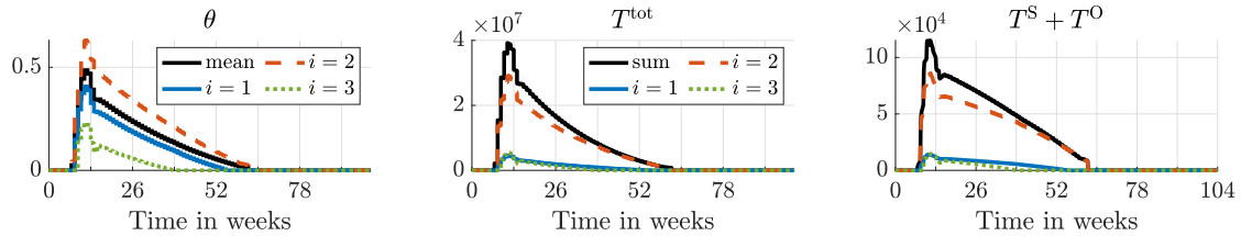
Figure 3: Optimal testing strategy for three age groups over two years.
