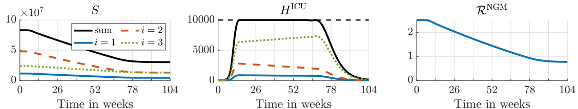
Figure 4: Evolution of the epidemic corresponding to the optimal testing strategy visualized in Figure 3 and reproduction number based on next-generation matrix. The dashed black line in the middle plot depicts the maximal capacity of ICUs.
