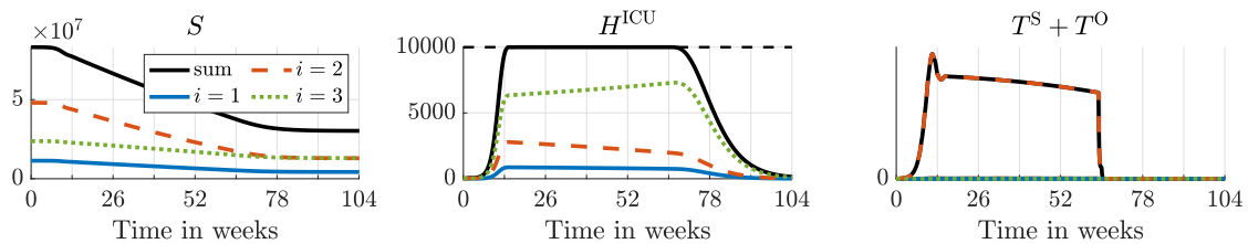
Figure 8: Evolution of the epidemic based on the controls visualized in Figure 7. The dashed black line in the plot of H^{\text{ICU}} depicts the upper bound on the number of available ICUs.
