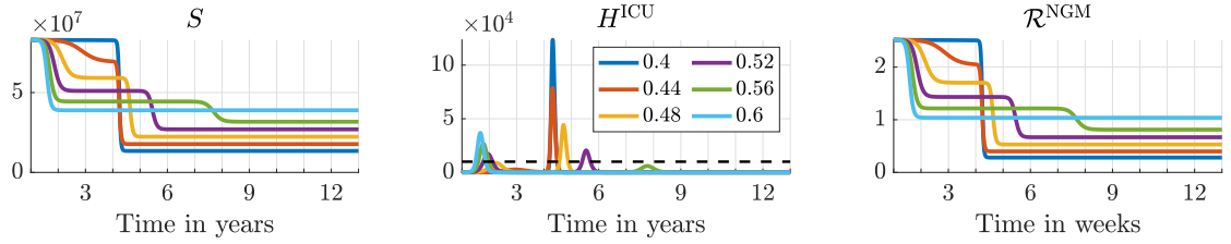
Figure 6: Solution for fixed \delta for three years and complete lift of restrictions afterwards.
