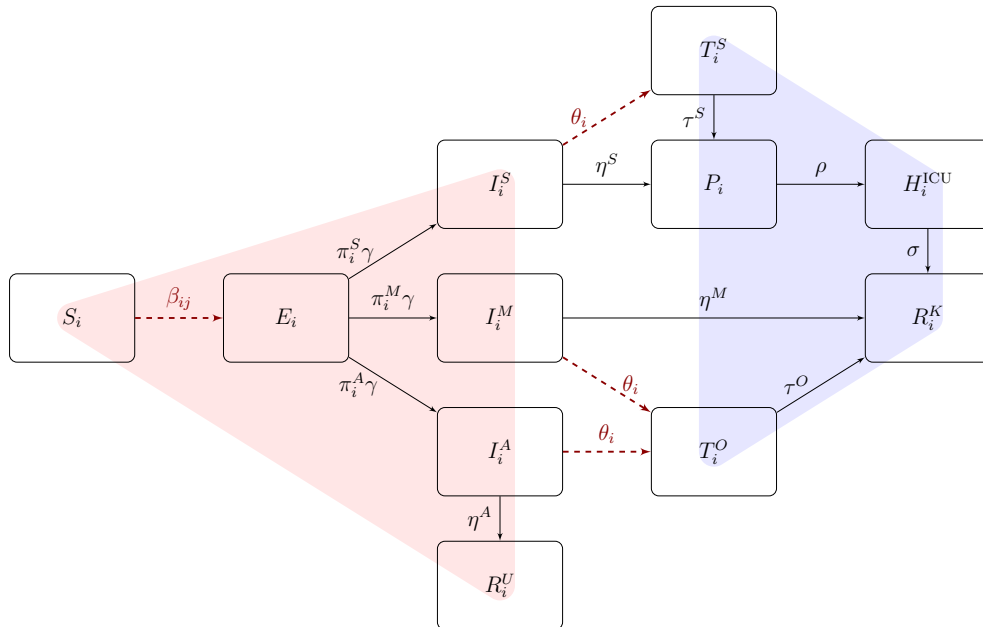
Figure 1: Flow of the SEITPHR model for one age group. The controls are indicated with dashed red edges. Unreported compartments are highlighted by the left red triangle, while tested and detected compartments are highlighted by the right blue trapezium.
