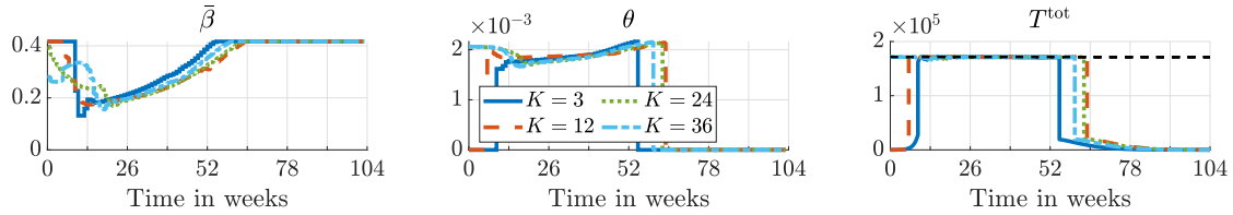
Figure 11: Optimal control for solving (8) in closed loop for varying prediction horizon length. For the sake of readability, we depicted average values of \theta and sums of T^{\text{tot}} over the age groups.
