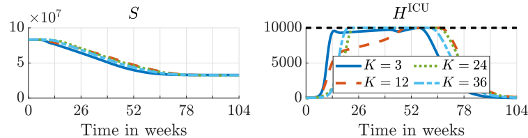
Figure 12: Evolution of the epidemic based on the controls depicted in Figure 11. For the sake of readability, only the sum over the age groups is visualized.
