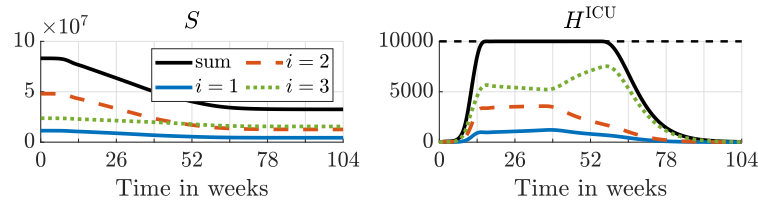
Figure 10: Evolution of the compartments associated with controls depicted in Figure 9.
