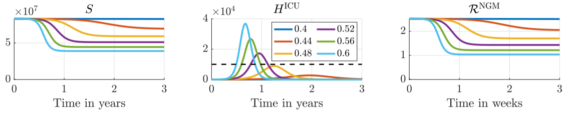
Figure 5: The impact of constant contact reduction rate \delta \in [0.4, 0.6] on the speed of evolution of the epidemic and on the number of required ICUs.
