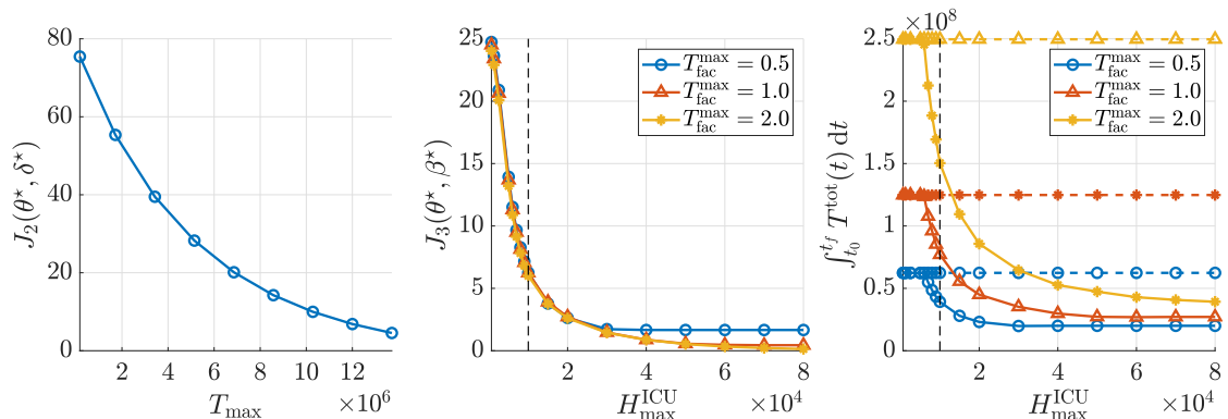
Figure 13: Impact of T^{\max} on social-distancing costs (left) and of H^{\max} on both social-distancing costs (middle) and testing (right). In the last two subfigures the currently available number of ICUs in Germany is highlighted by a vertical dashed line. The dashed horizontal lines in the right-most figure indicate the total testing capacities over the entire simulation horizon. Factor of modification of T^{\max} denoted by T_{\text{fac}}^{\max} .
