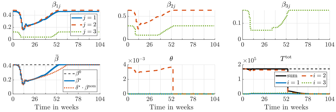
Figure 9: Optimal age-dependent social-distancing strategy for three age groups over two years.
