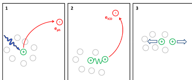
Figure 8. Experimental signatures of ICD. Left panel: ICD leads to a lifetime broadening of the excited state. This can be observed in the energy domain when the excited state is produced, for example, by photoionization or -excitation. Middle panel: Most obviously, the ICD electron can be observed directly. Right panel: The pair of ions created by ICD undergoes a Coulomb explosion. Detection of the final state ions also provides a strong indication for ICD. Experiments using these three characteristics have all been successfully performed in the past.
