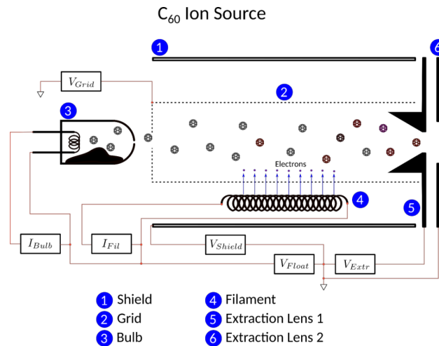
Figure 2.3: Schematic view of the C_{60} source.
